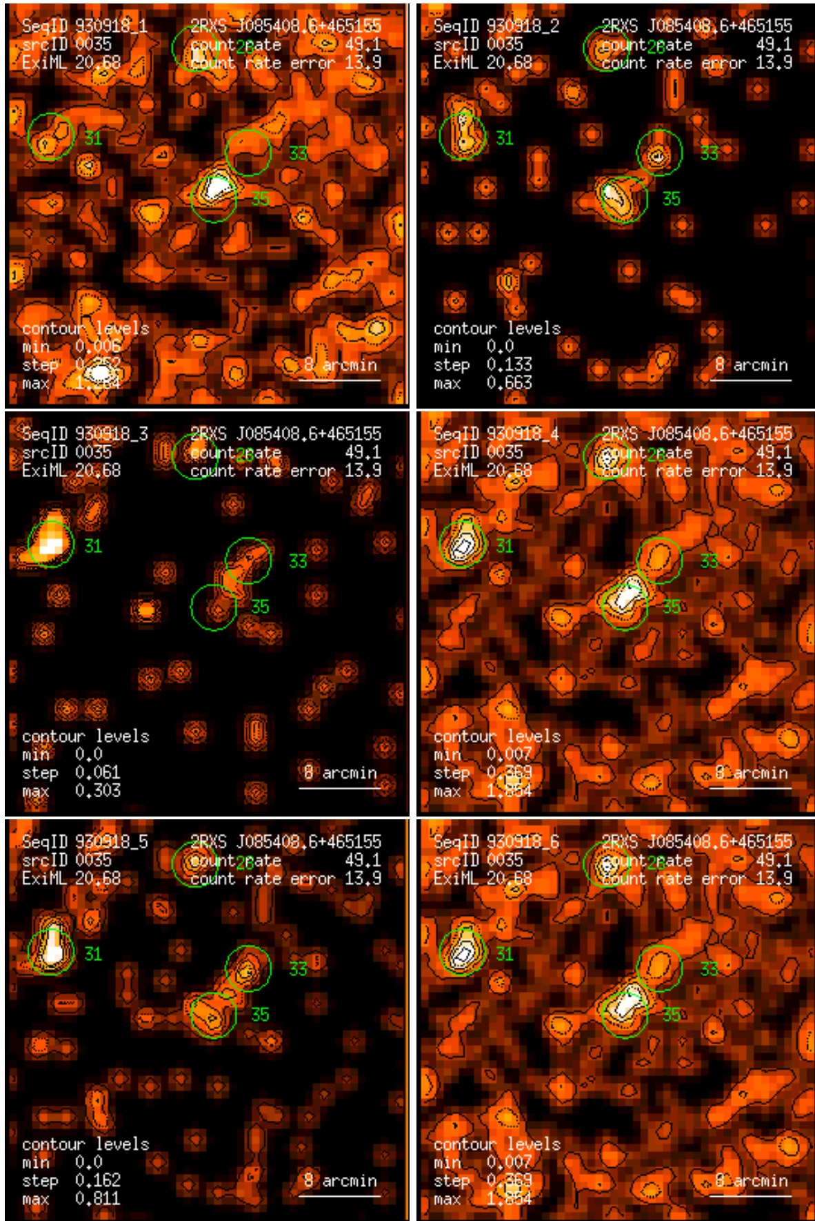
Figure 35: RASS 930918: detection 0035: band rate images, Gaussian filter: (1) PSPC channels 11 – 41, (2) 52 – 90, (3) 91 – 201, (4) 11 – 235, (5) 52 – 201, (6) 11 – 201. Broad band rates in counts/ks. Band rate contour levels in counts/ks/arcmin 2 .
