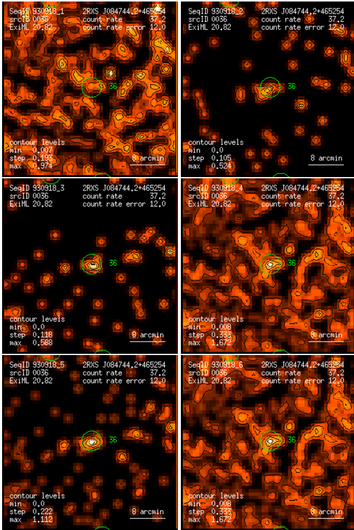
Figure 36: RASS 930918: detection 0036: band rate images, Gaussian filter: (1) PSPC channels 11 – 41, (2) 52 – 90, (3) 91 – 201, (4) 11 – 235, (5) 52 – 201, (6) 11 – 201. Broad band rates in counts/ks. Band rate contour levels in counts/ks/arcmin 2 .
