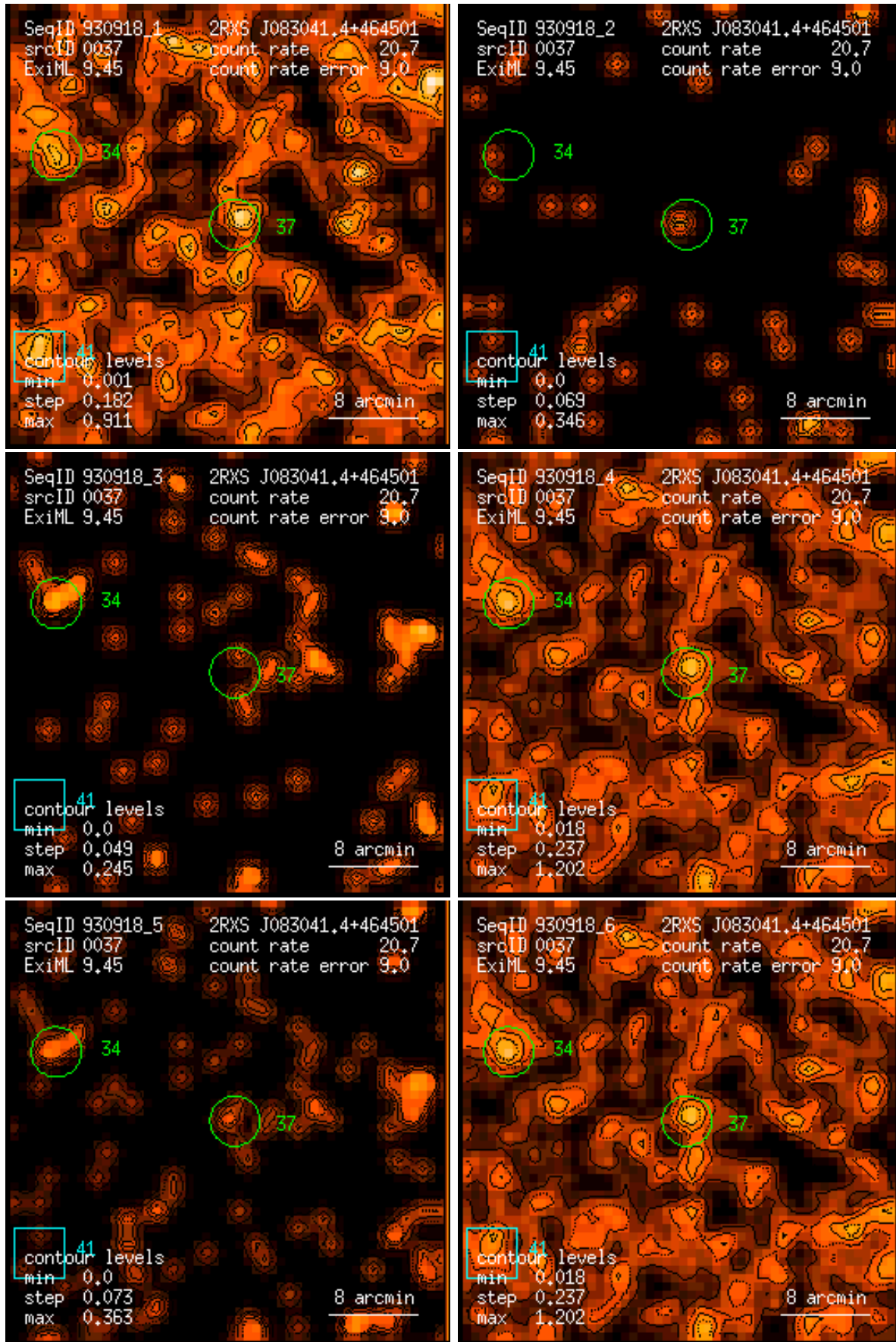
Figure 37: RASS 930918: detection 0037: band rate images, Gaussian filter: (1) PSPC channels 11 – 41, (2) 52 – 90, (3) 91 – 201, (4) 11 – 235, (5) 52 – 201, (6) 11 – 201. Broad band rates in counts/ks. Band rate contour levels in counts/ks/arcmin 2 .
