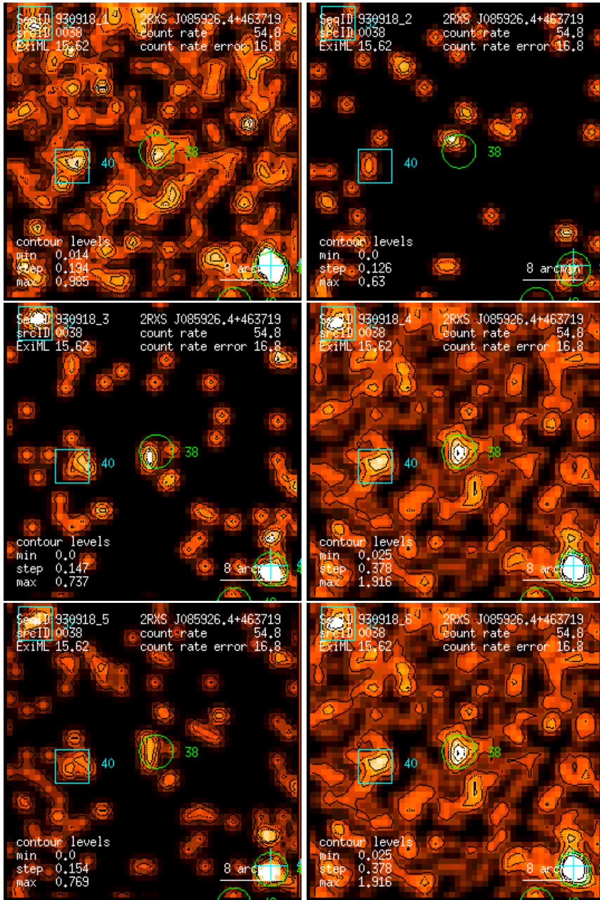
Figure 38: RASS 930918: detection 0038: band rate images, Gaussian filter: (1) PSPC channels 11 – 41, (2) 52 – 90, (3) 91 – 201, (4) 11 – 235, (5) 52 – 201, (6) 11 – 201. Broad band rates in counts/ks. Band rate contour levels in counts/ks/arcmin 2 .
