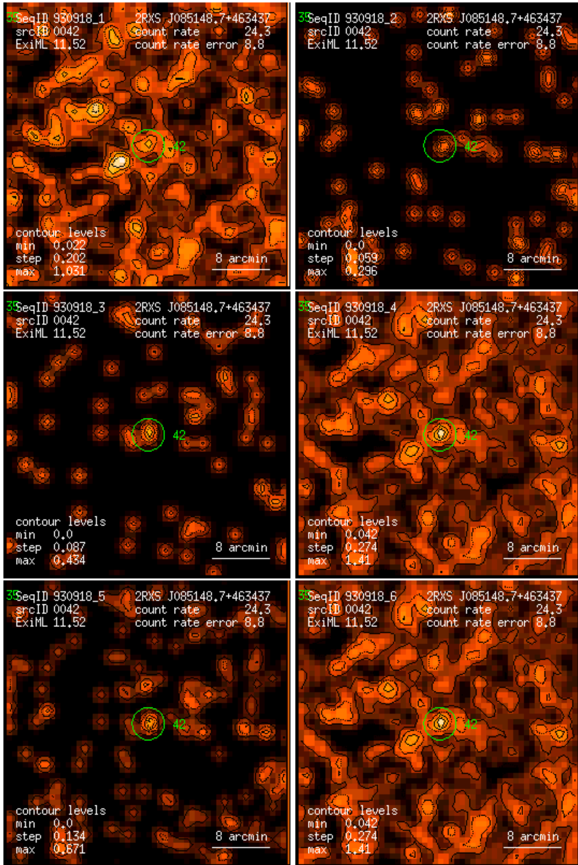
Figure 42: RASS 930918: detection 0042: band rate images, Gaussian filter: (1) PSPC channels 11 – 41, (2) 52 – 90, (3) 91 – 201, (4) 11 – 235, (5) 52 – 201, (6) 11 – 201. Broad band rates in counts/ks. Band rate contour levels in counts/ks/arcmin 2 .
