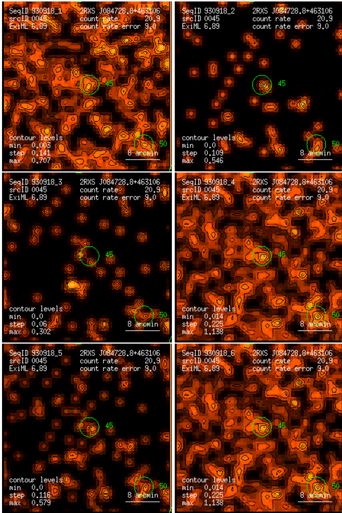
Figure 45: RASS 930918: detection 0045: band rate images, Gaussian filter: (1) PSPC channels 11 – 41, (2) 52 – 90, (3) 91 – 201, (4) 11 – 235, (5) 52 – 201, (6) 11 – 201. Broad band rates in counts/ks. Band rate contour levels in counts/ks/arcmin 2 .
