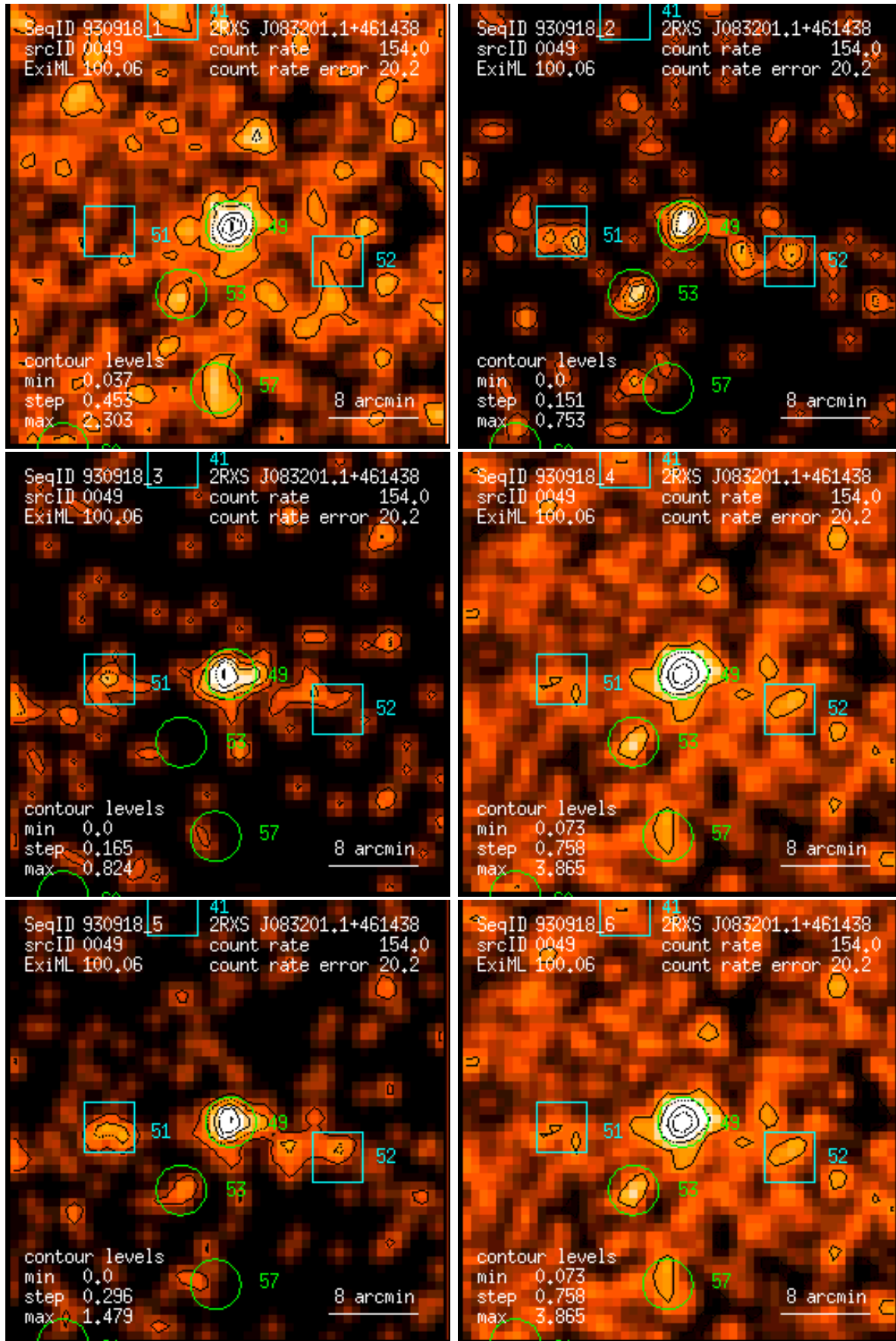
Figure 49: RASS 930918: detection 0049: band rate images, Gaussian filter: (1) PSPC channels 11 – 41, (2) 52 – 90, (3) 91 – 201, (4) 11 – 235, (5) 52 – 201, (6) 11 – 201. Broad band rates in counts/ks. Band rate contour levels in counts/ks/arcmin 2 .
