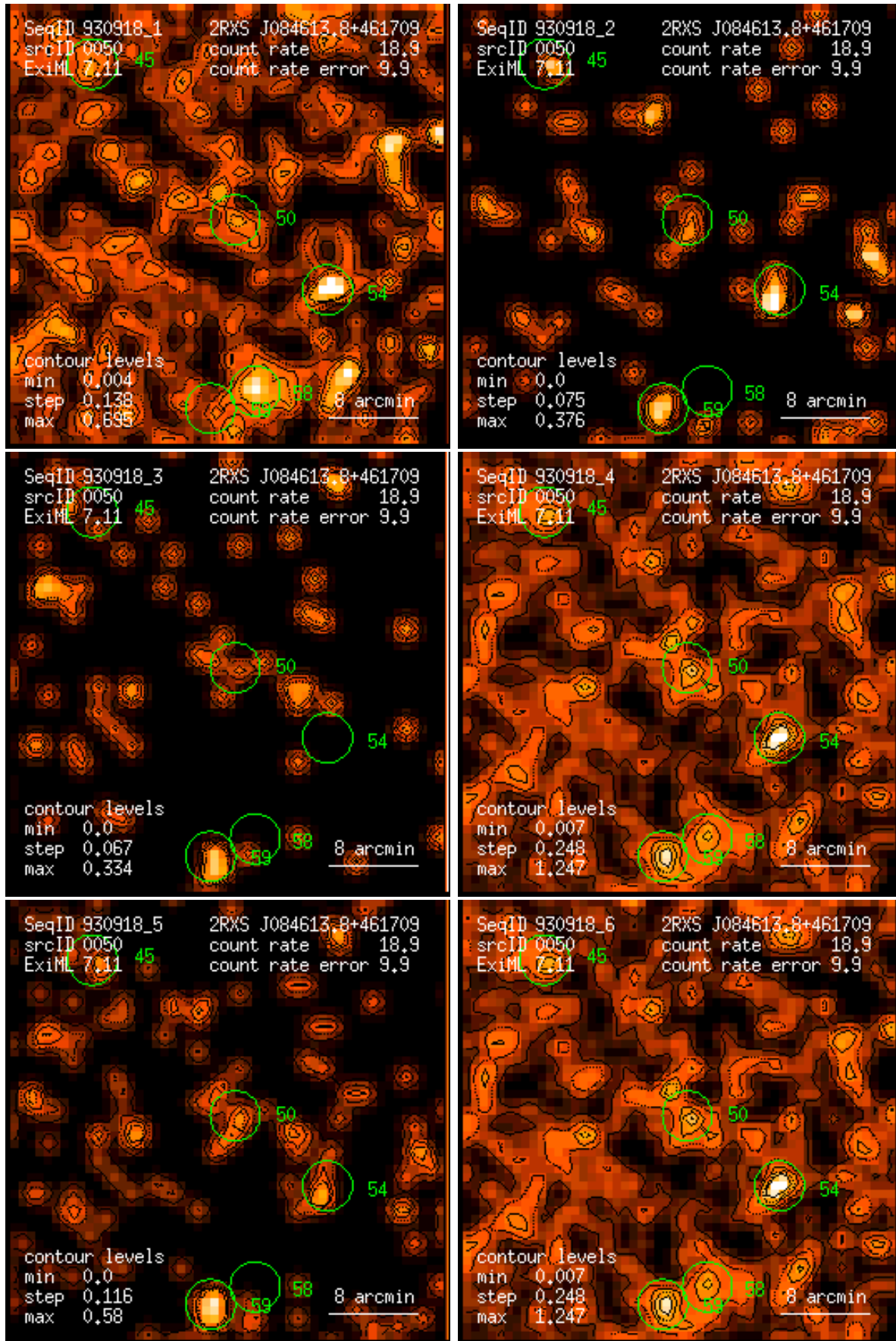
Figure 50: RASS 930918: detection 0050: band rate images, Gaussian filter: (1) PSPC channels 11 – 41, (2) 52 – 90, (3) 91 – 201, (4) 11 – 235, (5) 52 – 201, (6) 11 – 201. Broad band rates in counts/ks. Band rate contour levels in counts/ks/arcmin 2 .
