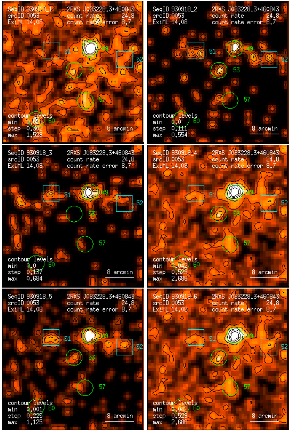
Figure 53: RASS 930918: detection 0053: band rate images, Gaussian filter: (1) PSPC channels 11 – 41, (2) 52 – 90, (3) 91 – 201, (4) 11 – 235, (5) 52 – 201, (6) 11 – 201. Broad band rates in counts/ks. Band rate contour levels in counts/ks/arcmin 2 .
