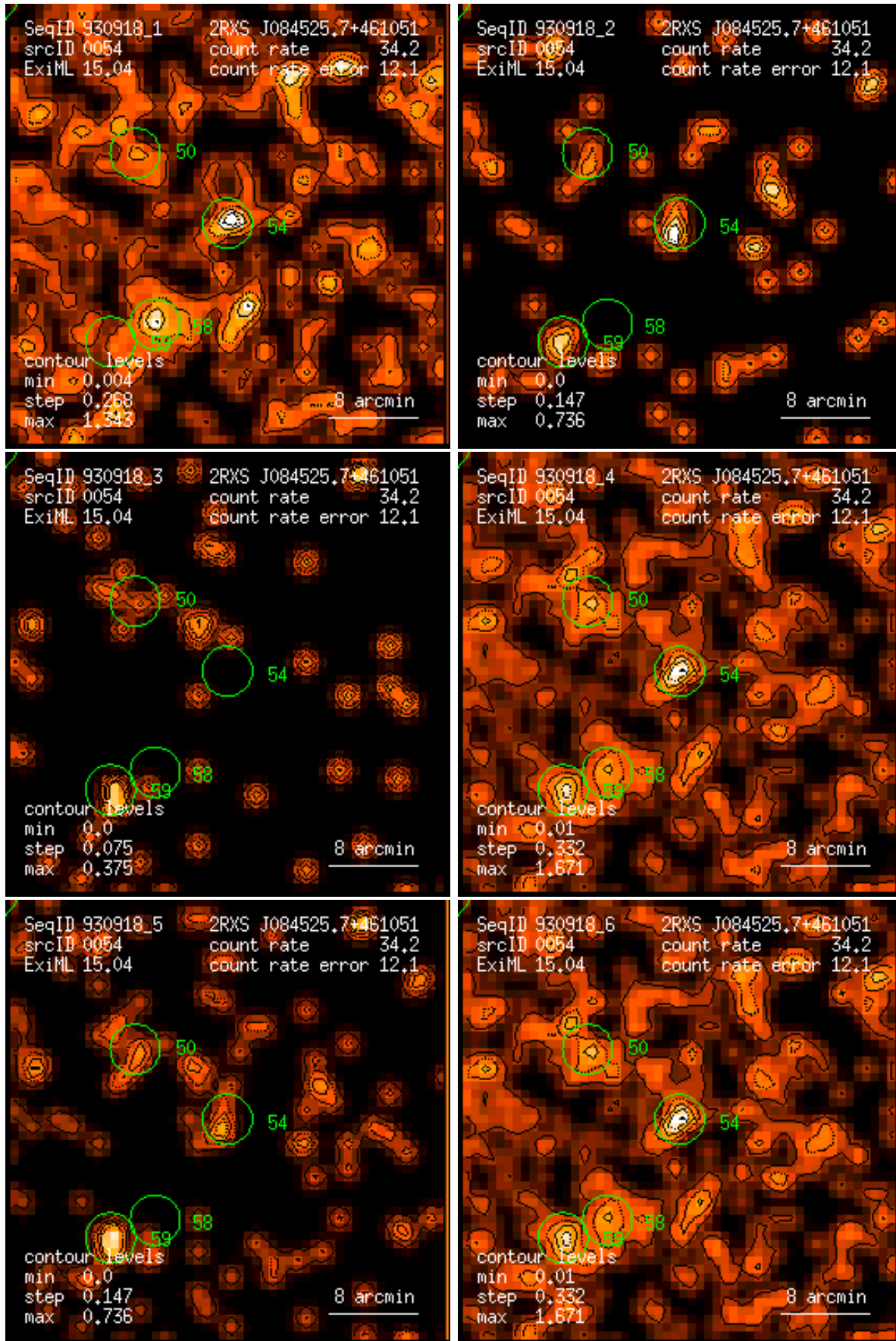
Figure 54: RASS 930918: detection 0054: band rate images, Gaussian filter: (1) PSPC channels 11 – 41, (2) 52 – 90, (3) 91 – 201, (4) 11 – 235, (5) 52 – 201, (6) 11 – 201. Broad band rates in counts/ks. Band rate contour levels in counts/ks/arcmin 2 .
