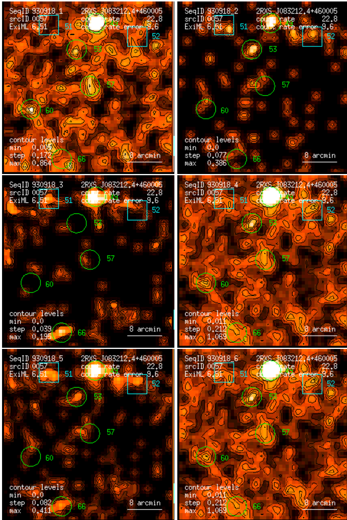
Figure 57: RASS 930918: detection 0057: band rate images, Gaussian filter: (1) PSPC channels 11 – 41, (2) 52 – 90, (3) 91 – 201, (4) 11 – 235, (5) 52 – 201, (6) 11 – 201. Broad band rates in counts/ks. Band rate contour levels in counts/ks/arcmin 2 .
