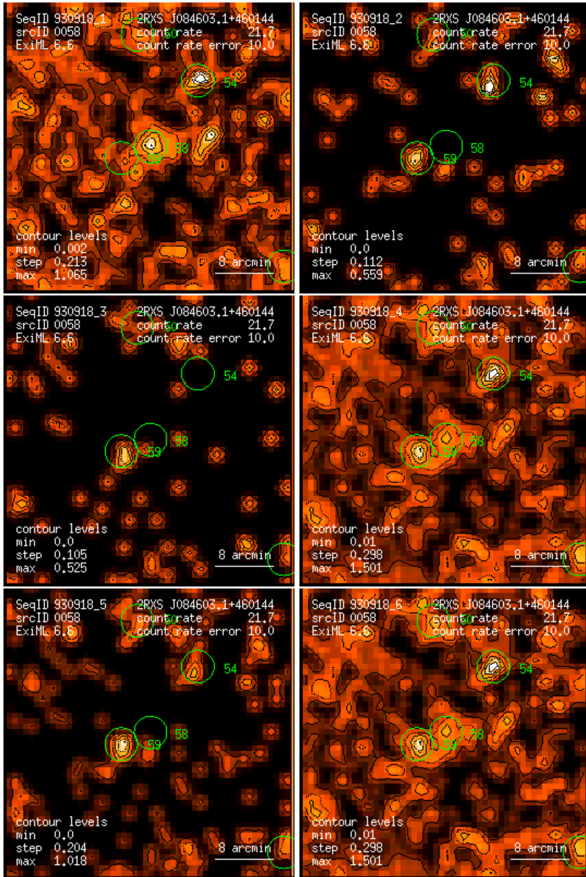
Figure 58: RASS 930918: detection 0058: band rate images, Gaussian filter: (1) PSPC channels 11 – 41, (2) 52 – 90, (3) 91 – 201, (4) 11 – 235, (5) 52 – 201, (6) 11 – 201. Broad band rates in counts/ks. Band rate contour levels in counts/ks/arcmin 2 .
