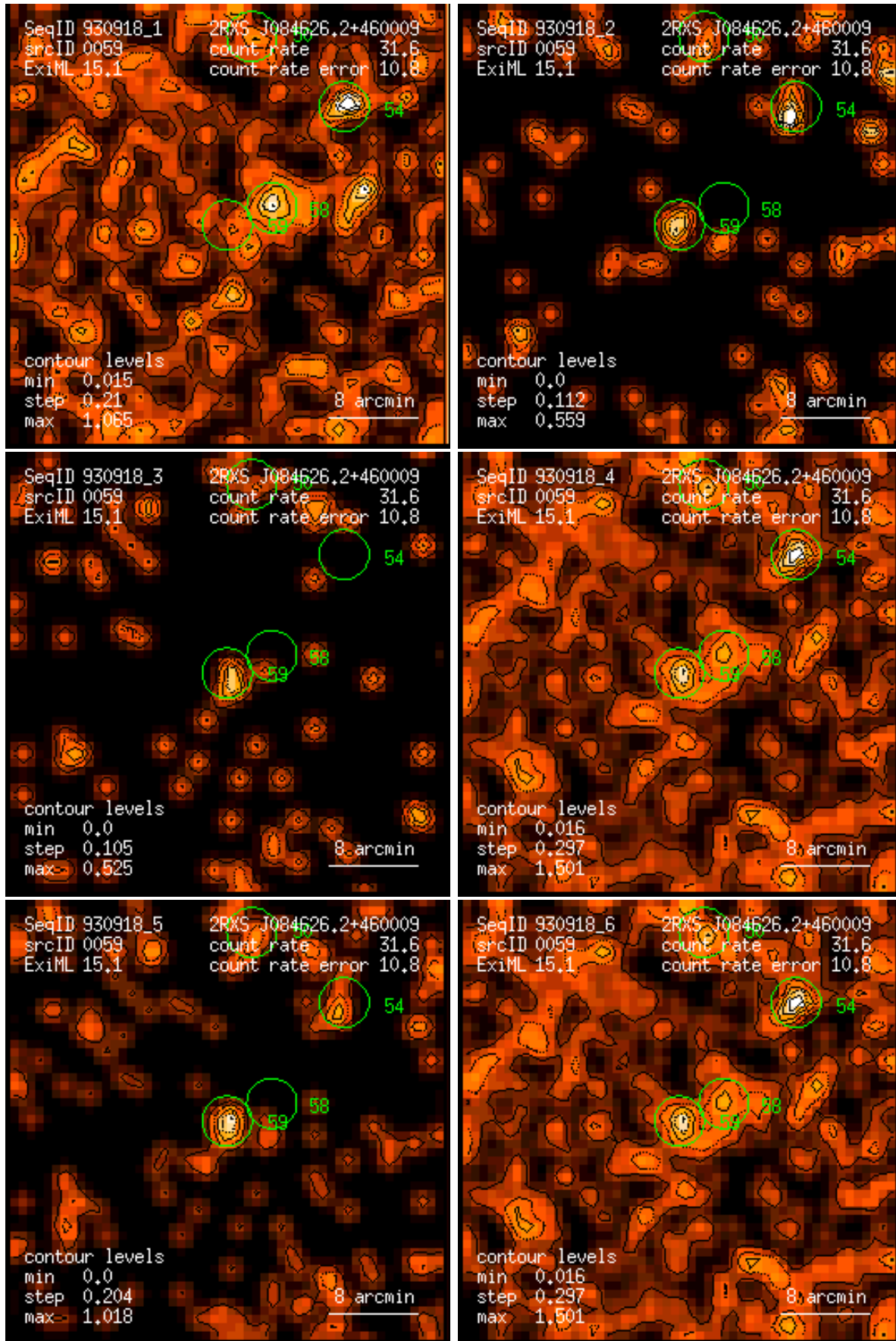
Figure 59: RASS 930918: detection 0059: band rate images, Gaussian filter: (1) PSPC channels 11 – 41, (2) 52 – 90, (3) 91 – 201, (4) 11 – 235, (5) 52 – 201, (6) 11 – 201. Broad band rates in counts/ks. Band rate contour levels in counts/ks/arcmin 2 .
