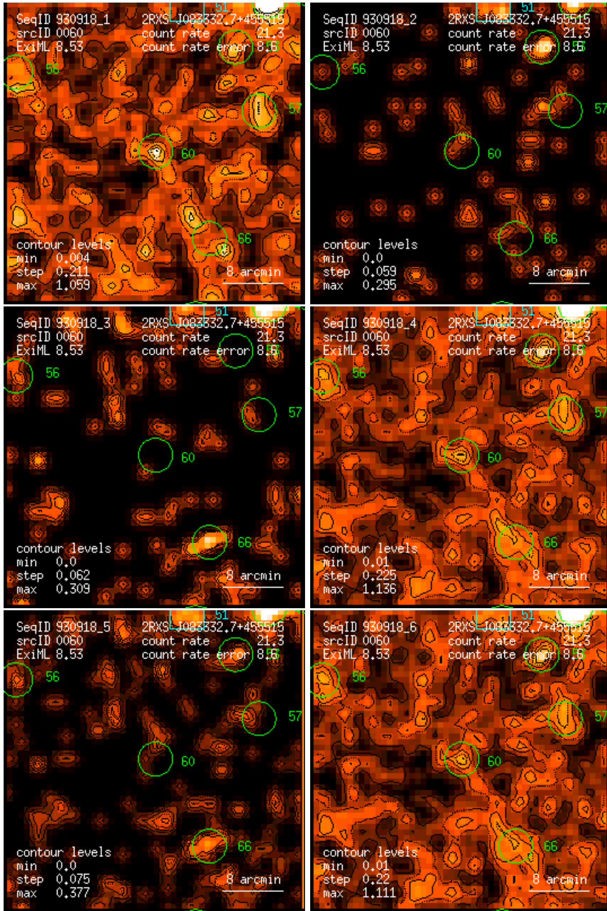
Figure 60: RASS 930918: detection 0060: band rate images, Gaussian filter: (1) PSPC channels 11 – 41, (2) 52 – 90, (3) 91 – 201, (4) 11 – 235, (5) 52 – 201, (6) 11 – 201. Broad band rates in counts/ks. Band rate contour levels in counts/ks/arcmin 2 .
