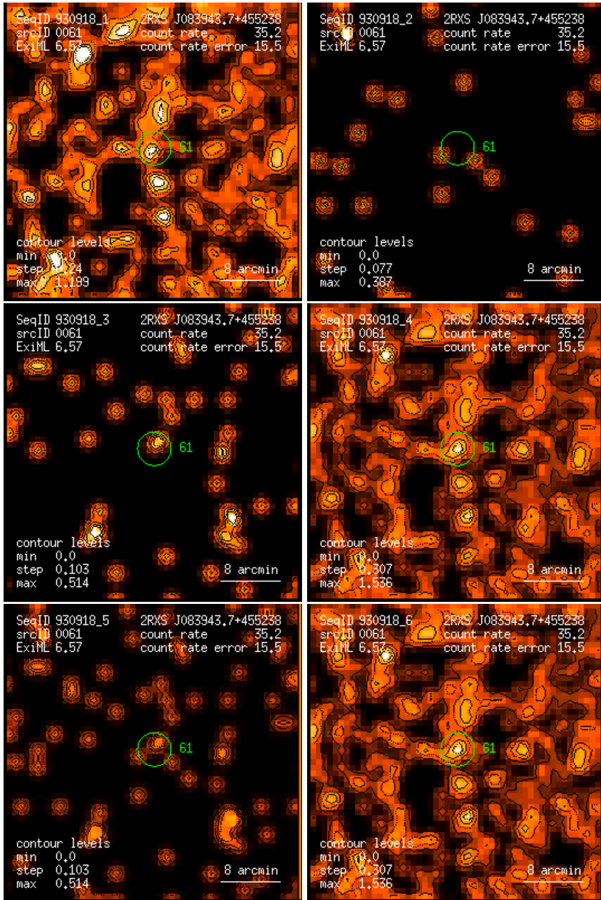
Figure 61: RASS 930918: detection 0061: band rate images, Gaussian filter: (1) PSPC channels 11 – 41, (2) 52 – 90, (3) 91 – 201, (4) 11 – 235, (5) 52 – 201, (6) 11 – 201. Broad band rates in counts/ks. Band rate contour levels in counts/ks/arcmin 2 .
