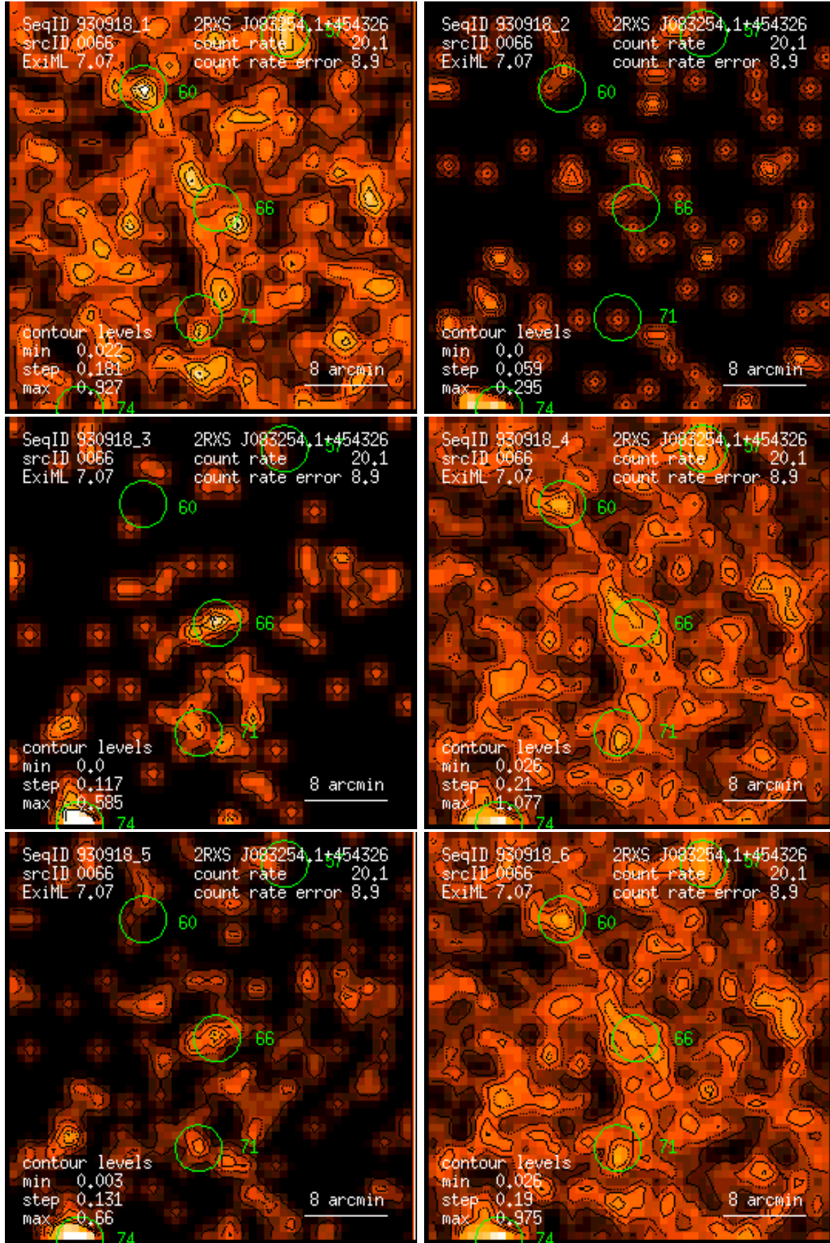
Figure 66: RASS 930918: detection 0066: band rate images, Gaussian filter: (1) PSPC channels 11 – 41, (2) 52 – 90, (3) 91 – 201, (4) 11 – 235, (5) 52 – 201, (6) 11 – 201. Broad band rates in counts/ks. Band rate contour levels in counts/ks/arcmin 2 .
