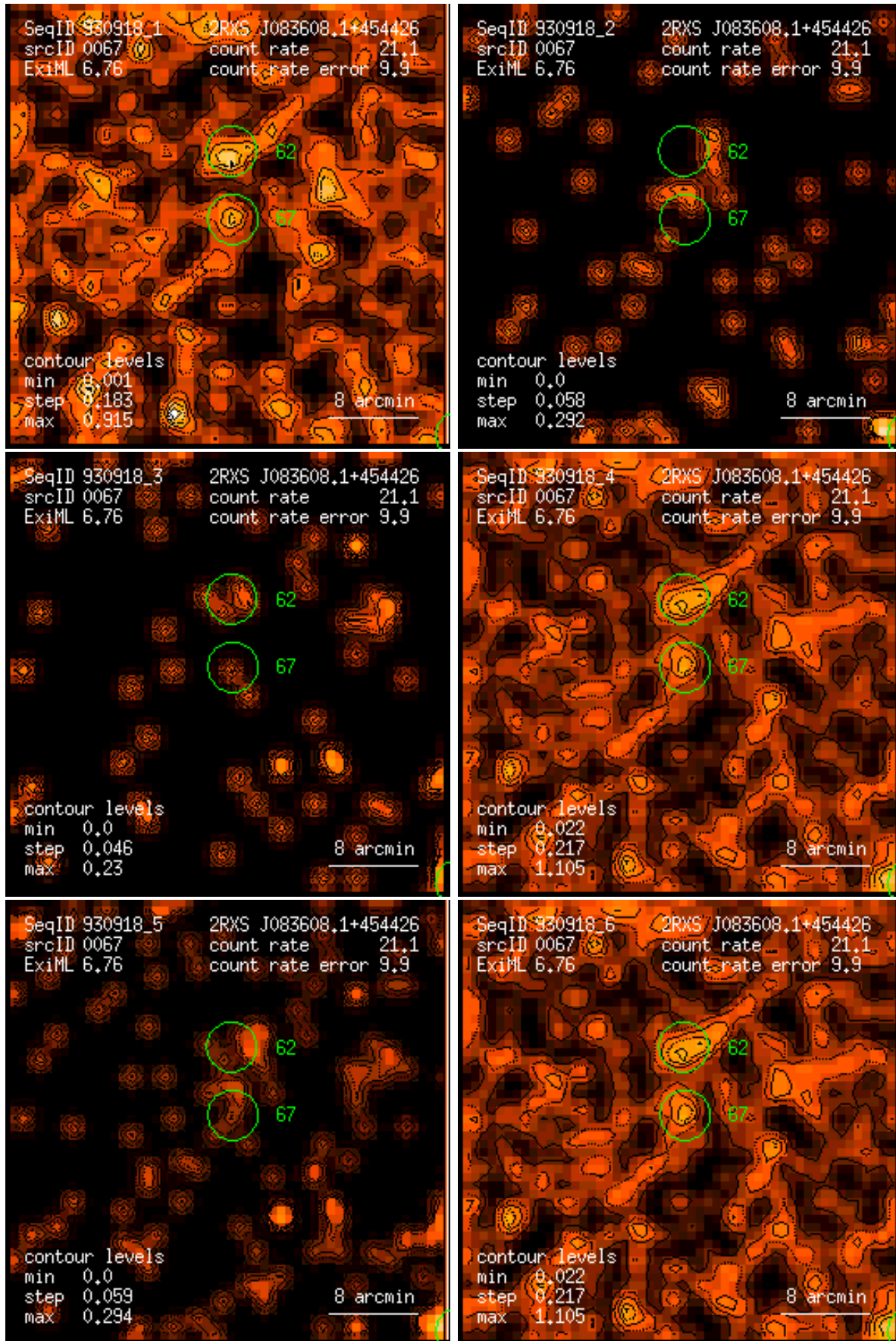
Figure 67: RASS 930918: detection 0067: band rate images, Gaussian filter: (1) PSPC channels 11 – 41, (2) 52 – 90, (3) 91 – 201, (4) 11 – 235, (5) 52 – 201, (6) 11 – 201. Broad band rates in counts/ks. Band rate contour levels in counts/ks/arcmin 2 .
