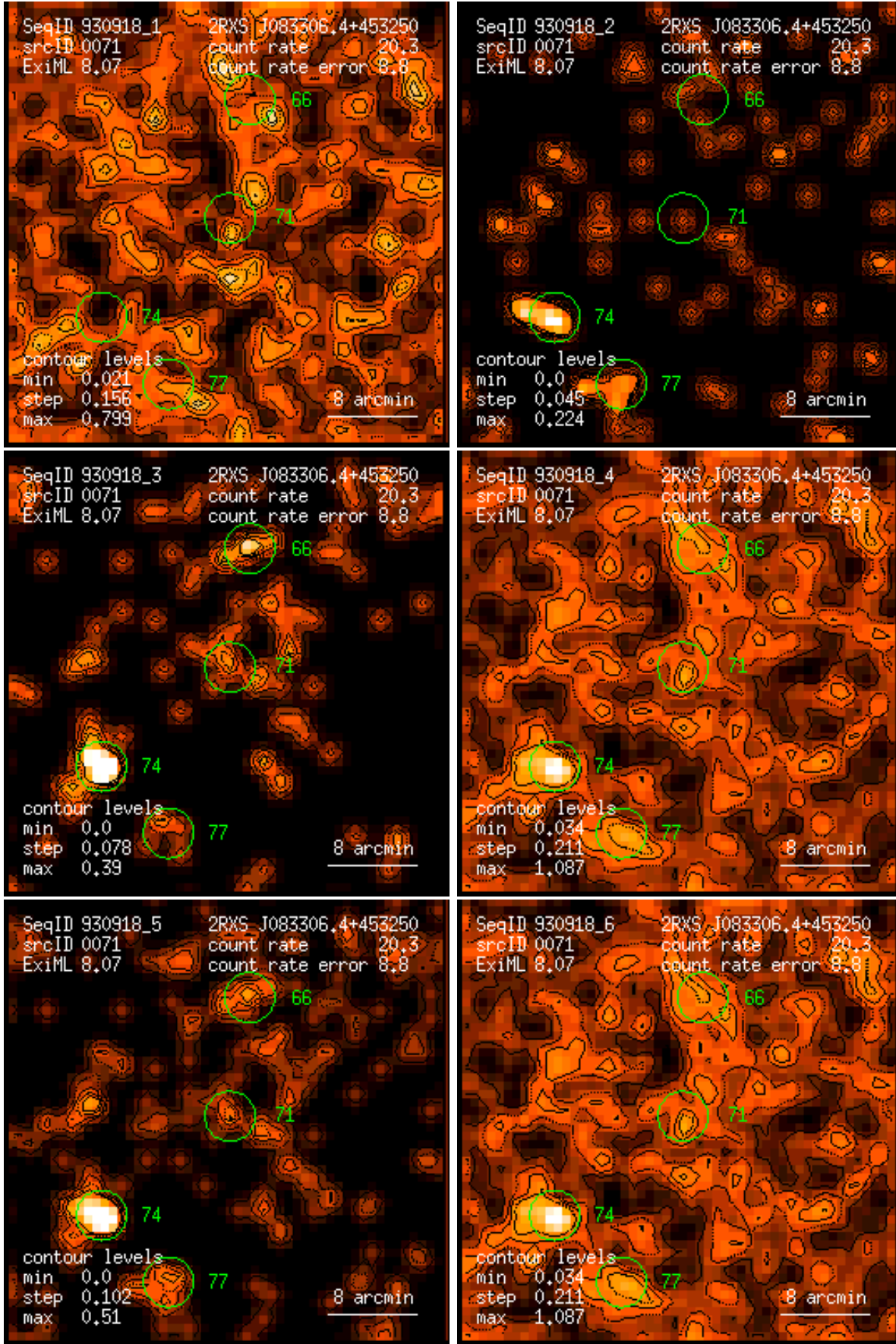
Figure 71: RASS 930918: detection 0071: band rate images, Gaussian filter: (1) PSPC channels 11 – 41, (2) 52 – 90, (3) 91 – 201, (4) 11 – 235, (5) 52 – 201, (6) 11 – 201. Broad band rates in counts/ks. Band rate contour levels in counts/ks/arcmin 2 .
