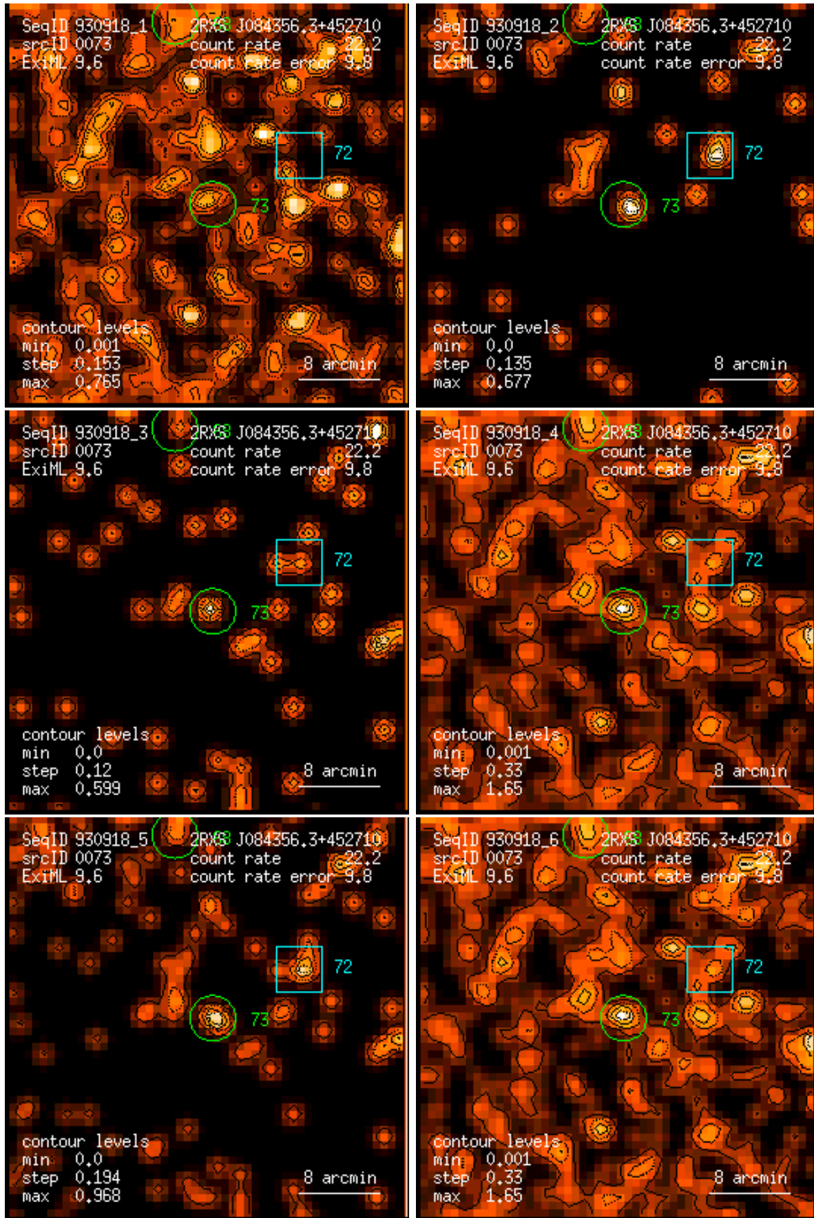
Figure 73: RASS 930918: detection 0073: band rate images, Gaussian filter: (1) PSPC channels 11 – 41, (2) 52 – 90, (3) 91 – 201, (4) 11 – 235, (5) 52 – 201, (6) 11 – 201. Broad band rates in counts/ks. Band rate contour levels in counts/ks/arcmin 2 .
