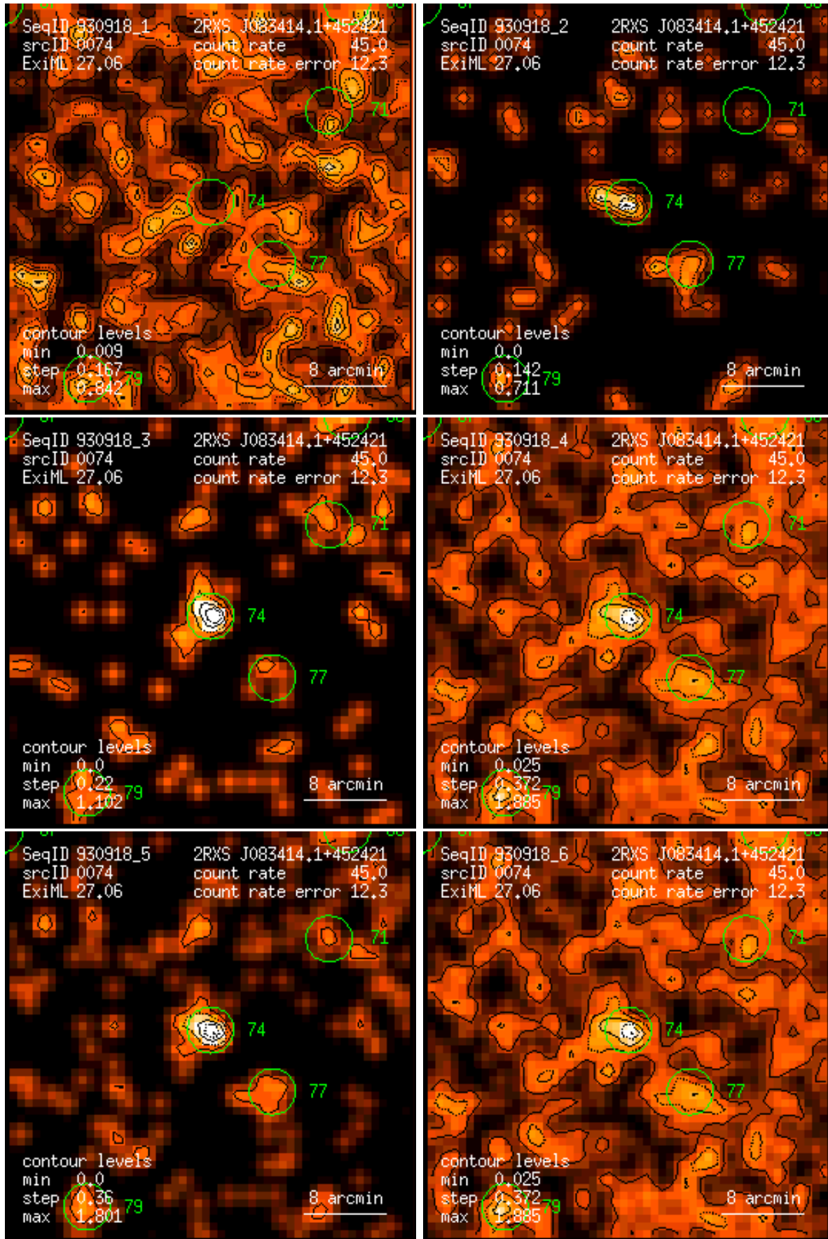
Figure 74: RASS 930918: detection 0074: band rate images, Gaussian filter: (1) PSPC channels 11 – 41, (2) 52 – 90, (3) 91 – 201, (4) 11 – 235, (5) 52 – 201, (6) 11 – 201. Broad band rates in counts/ks. Band rate contour levels in counts/ks/arcmin 2 .
