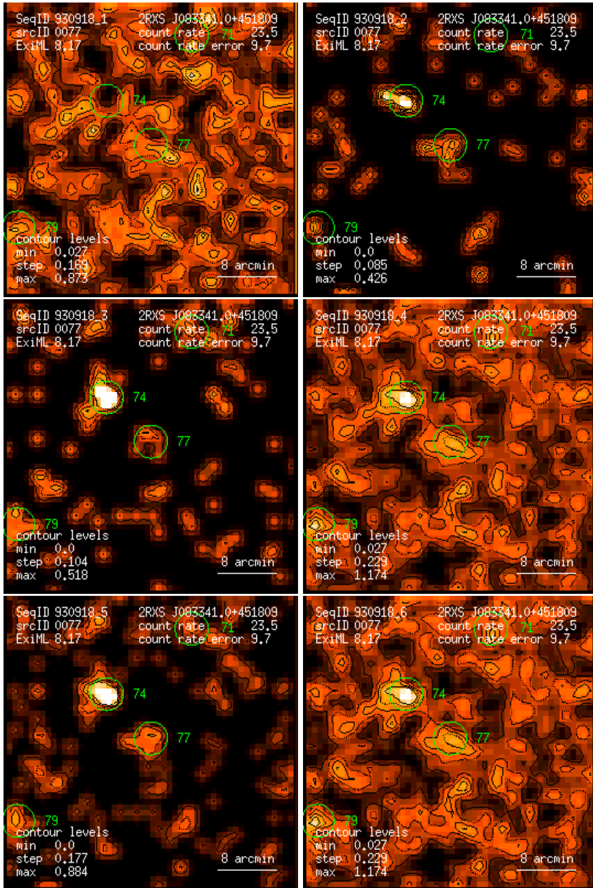
Figure 77: RASS 930918: detection 0077: band rate images, Gaussian filter: (1) PSPC channels 11 – 41, (2) 52 – 90, (3) 91 – 201, (4) 11 – 235, (5) 52 – 201, (6) 11 – 201. Broad band rates in counts/ks. Band rate contour levels in counts/ks/arcmin 2 .
