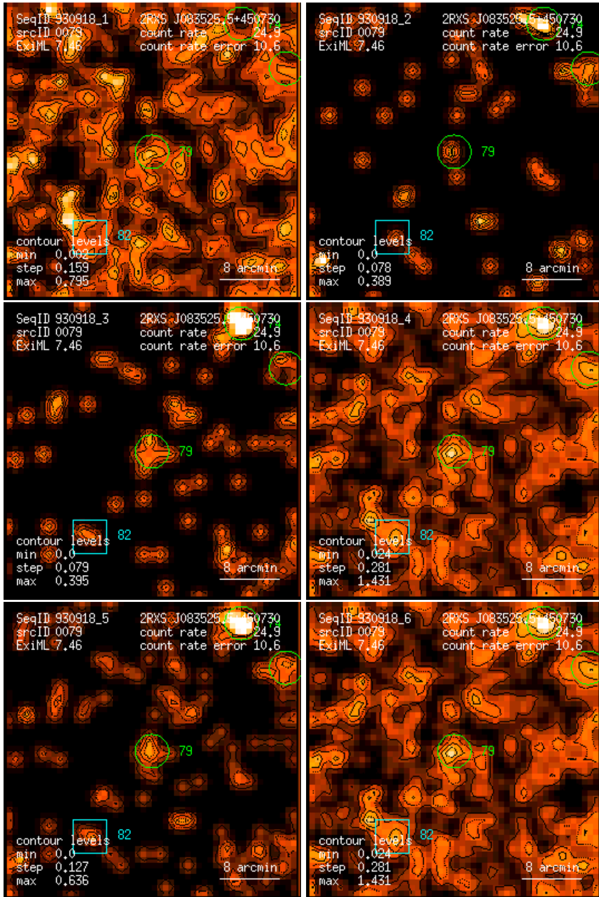
Figure 79: RASS 930918: detection 0079: band rate images, Gaussian filter: (1) PSPC channels 11 – 41, (2) 52 – 90, (3) 91 – 201, (4) 11 – 235, (5) 52 – 201, (6) 11 – 201. Broad band rates in counts/ks. Band rate contour levels in counts/ks/arcmin 2 .
