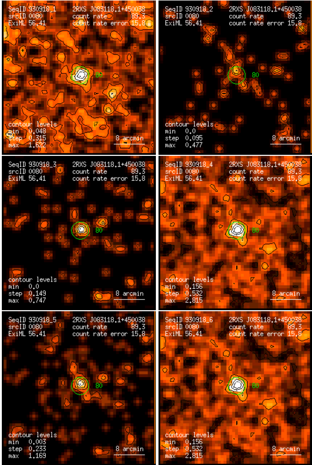
Figure 80: RASS 930918: detection 0080: band rate images, Gaussian filter: (1) PSPC channels 11 – 41, (2) 52 – 90, (3) 91 – 201, (4) 11 – 235, (5) 52 – 201, (6) 11 – 201. Broad band rates in counts/ks. Band rate contour levels in counts/ks/arcmin 2 .
