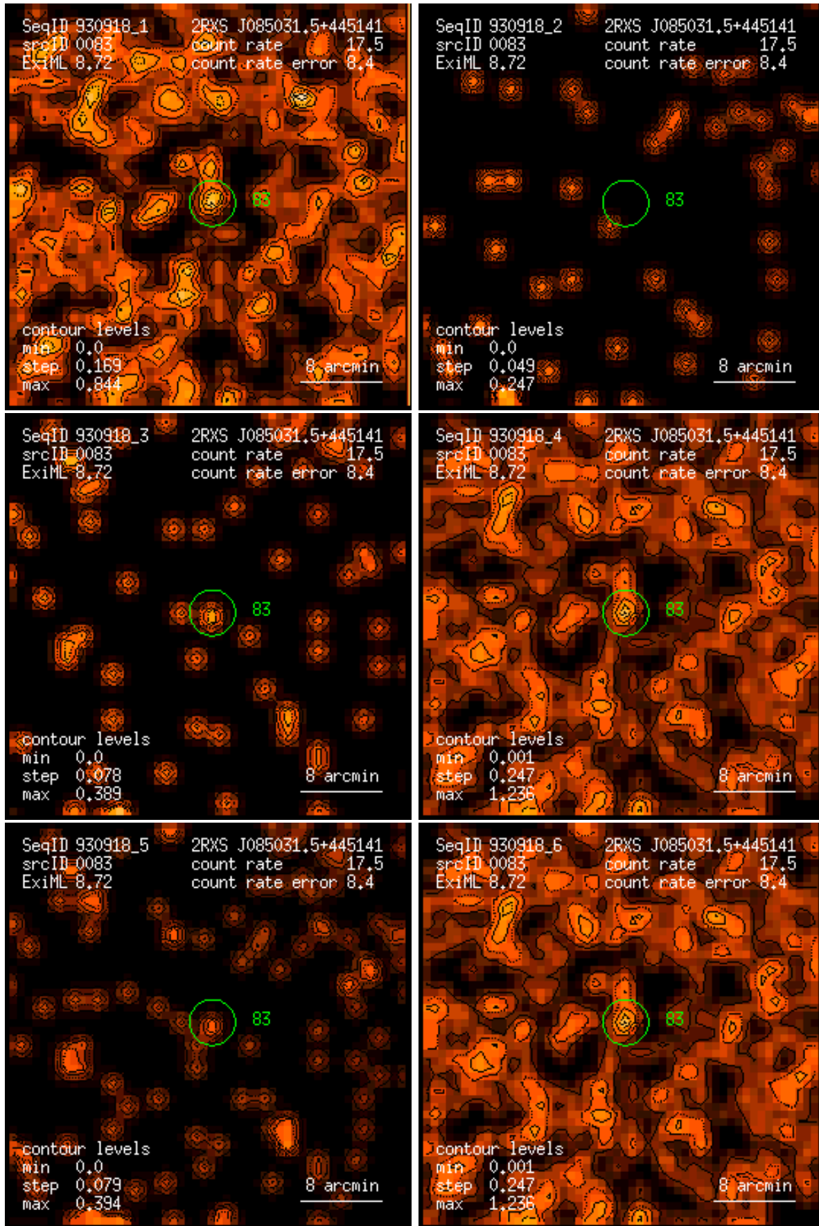
Figure 83: RASS 930918: detection 0083: band rate images, Gaussian filter: (1) PSPC channels 11 – 41, (2) 52 – 90, (3) 91 – 201, (4) 11 – 235, (5) 52 – 201, (6) 11 – 201. Broad band rates in counts/ks. Band rate contour levels in counts/ks/arcmin 2 .
