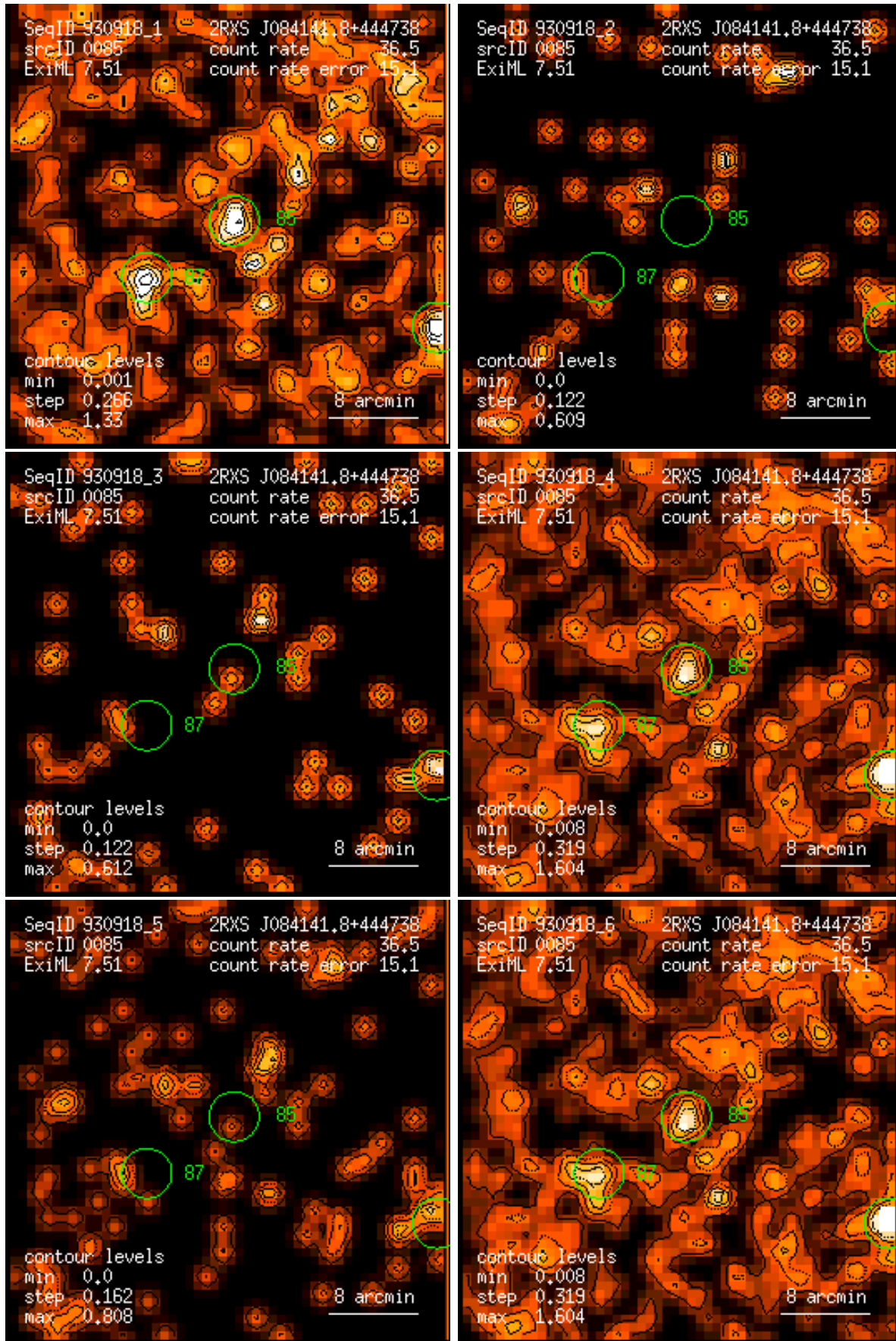
Figure 85: RASS 930918: detection 0085: band rate images, Gaussian filter: (1) PSPC channels 11 – 41, (2) 52 – 90, (3) 91 – 201, (4) 11 – 235, (5) 52 – 201, (6) 11 – 201. Broad band rates in counts/ks. Band rate contour levels in counts/ks/arcmin 2 .
