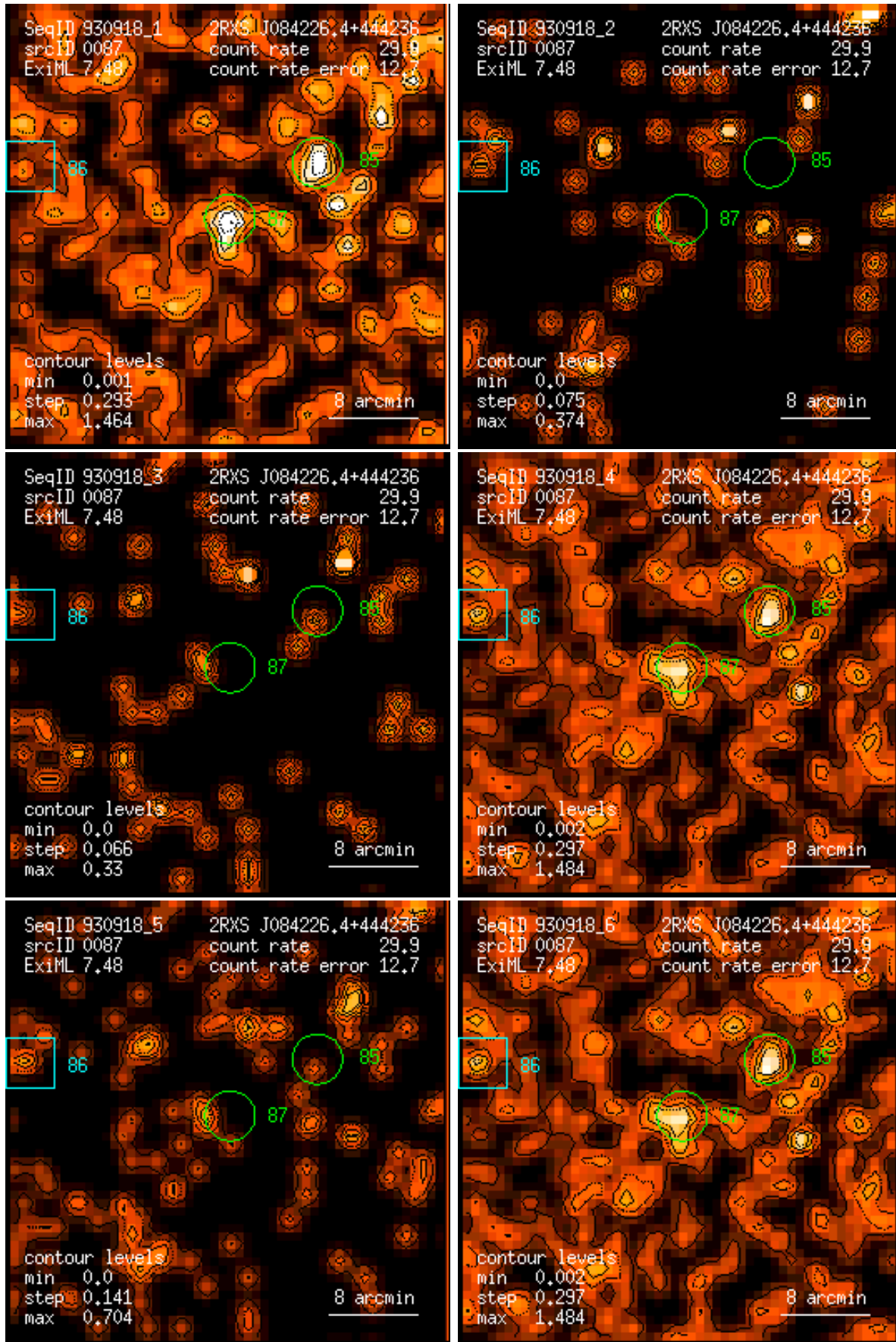
Figure 87: RASS 930918: detection 0087: band rate images, Gaussian filter: (1) PSPC channels 11 – 41, (2) 52 – 90, (3) 91 – 201, (4) 11 – 235, (5) 52 – 201, (6) 11 – 201. Broad band rates in counts/ks. Band rate contour levels in counts/ks/arcmin 2 .
