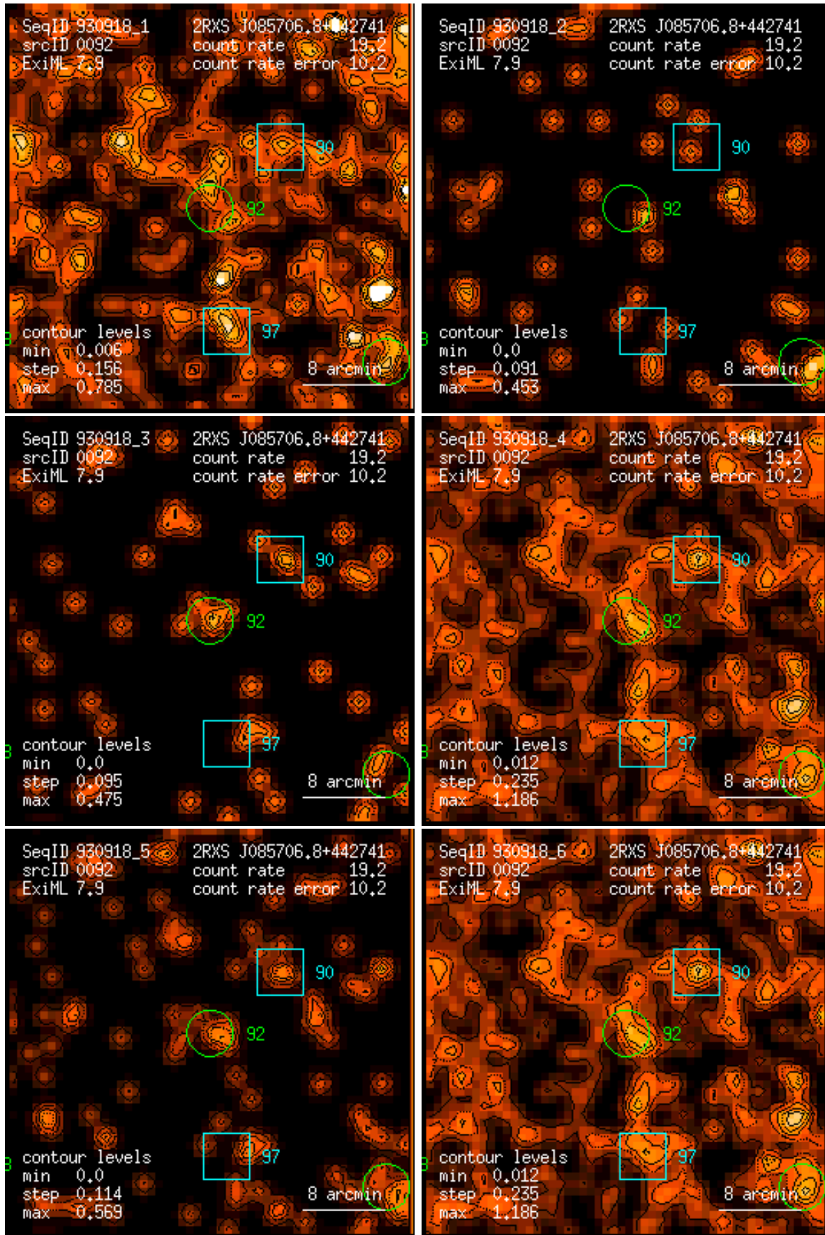
Figure 92: RASS 930918: detection 0092: band rate images, Gaussian filter: (1) PSPC channels 11 – 41, (2) 52 – 90, (3) 91 – 201, (4) 11 – 235, (5) 52 – 201, (6) 11 – 201. Broad band rates in counts/ks. Band rate contour levels in counts/ks/arcmin 2 .
