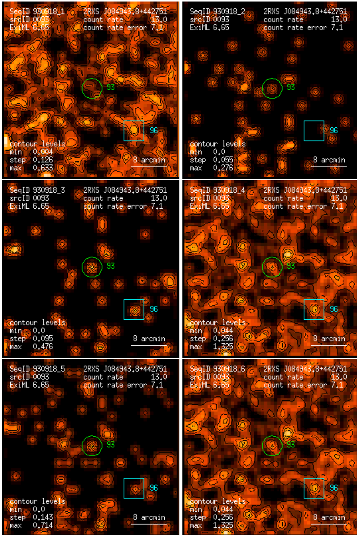
Figure 93: RASS 930918: detection 0093: band rate images, Gaussian filter: (1) PSPC channels 11 – 41, (2) 52 – 90, (3) 91 – 201, (4) 11 – 235, (5) 52 – 201, (6) 11 – 201. Broad band rates in counts/ks. Band rate contour levels in counts/ks/arcmin 2 .
