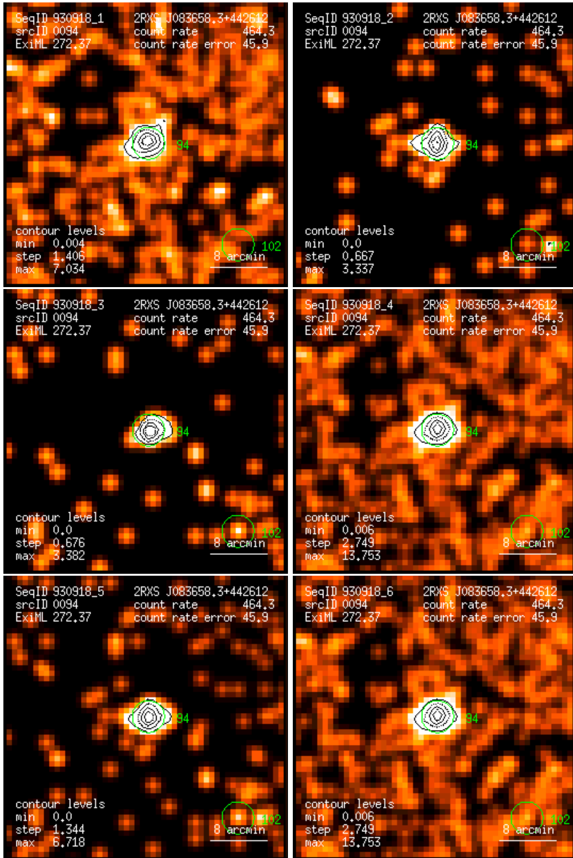
Figure 94: RASS 930918: detection 0094: band rate images, Gaussian filter: (1) PSPC channels 11 – 41, (2) 52 – 90, (3) 91 – 201, (4) 11 – 235, (5) 52 – 201, (6) 11 – 201. Broad band rates in counts/ks. Band rate contour levels in counts/ks/arcmin 2 .
