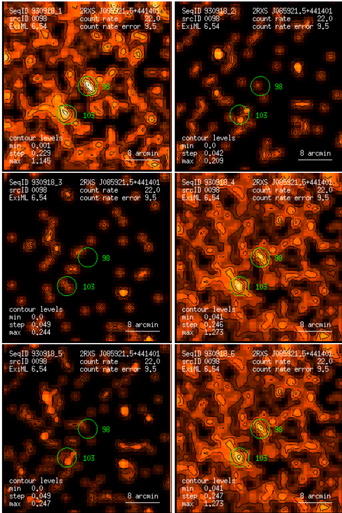
Figure 98: RASS 930918: detection 0098: band rate images, Gaussian filter: (1) PSPC channels 11 – 41, (2) 52 – 90, (3) 91 – 201, (4) 11 – 235, (5) 52 – 201, (6) 11 – 201. Broad band rates in counts/ks. Band rate contour levels in counts/ks/arcmin 2 .
