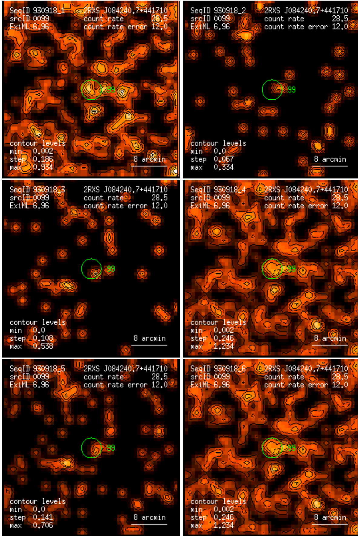
Figure 99: RASS 930918: detection 0099: band rate images, Gaussian filter: (1) PSPC channels 11 – 41, (2) 52 – 90, (3) 91 – 201, (4) 11 – 235, (5) 52 – 201, (6) 11 – 201. Broad band rates in counts/ks. Band rate contour levels in counts/ks/arcmin 2 .
