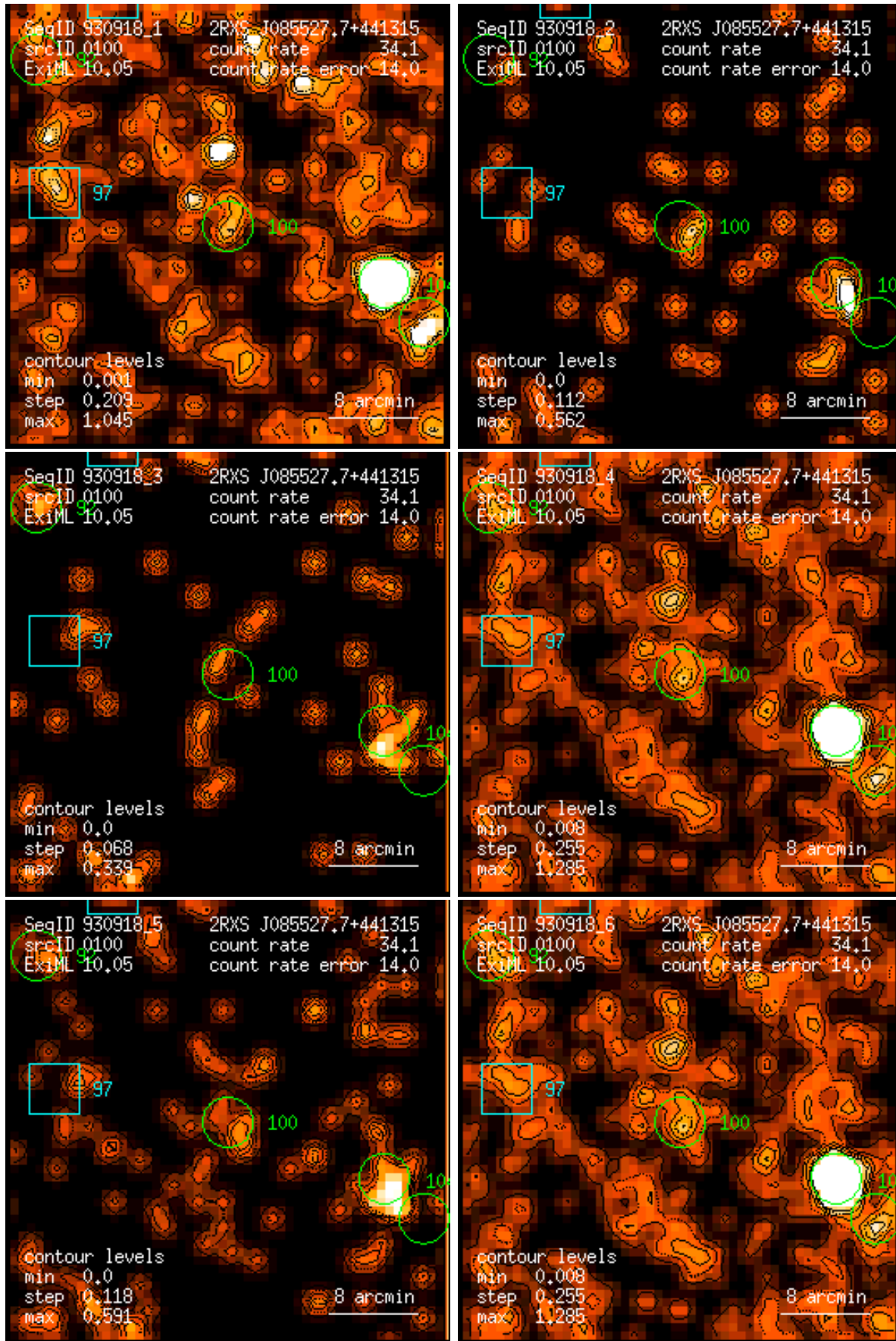
Figure 100: RASS 930918: detection 0100: band rate images, Gaussian filter: (1) PSPC channels 11 – 41, (2) 52 – 90, (3) 91 – 201, (4) 11 – 235, (5) 52 – 201, (6) 11 – 201. Broad band rates in counts/ks. Band rate contour levels in counts/ks/arcmin 2 .
