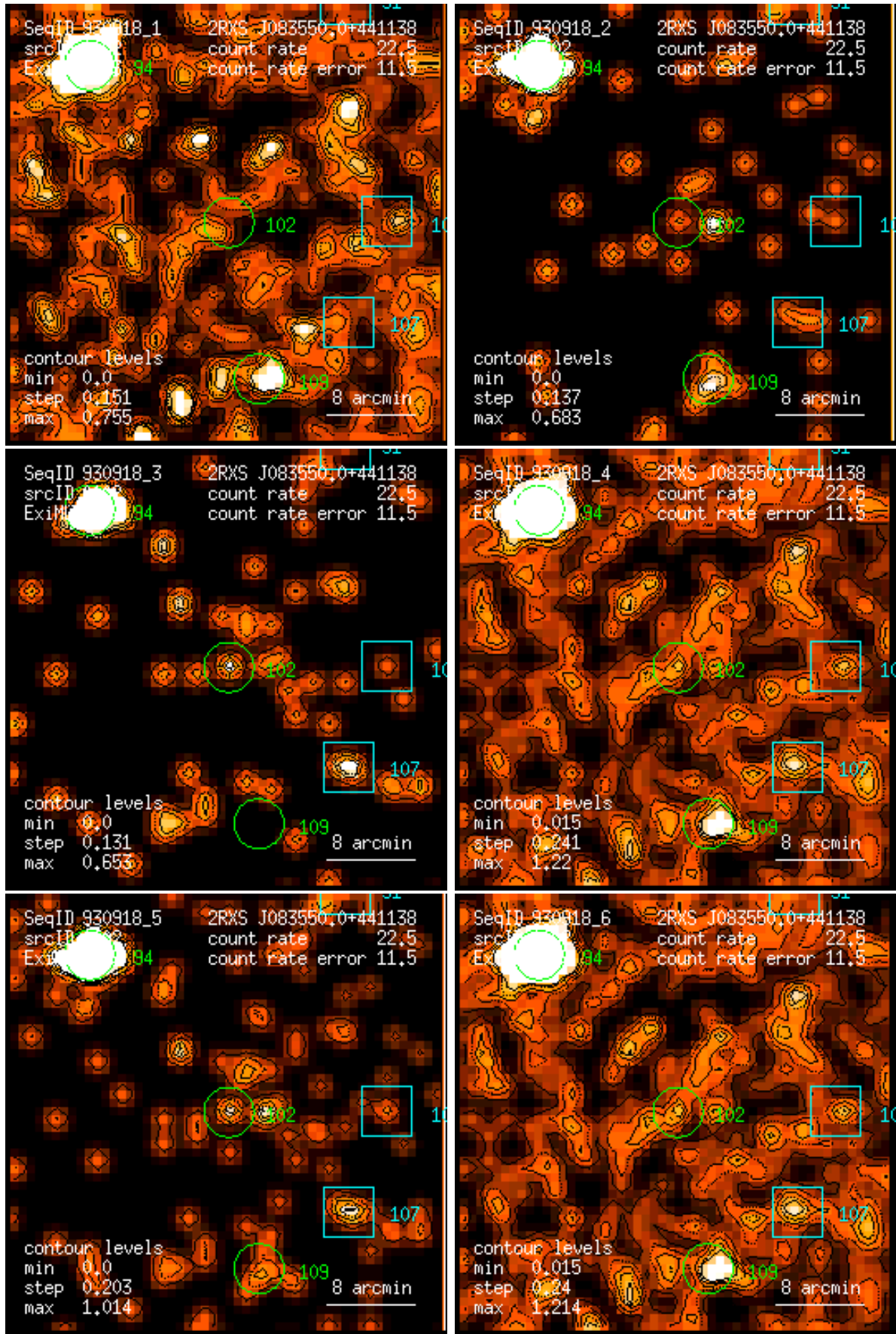
Figure 102: RASS 930918: detection 0102: band rate images, Gaussian filter: (1) PSPC channels 11 – 41, (2) 52 – 90, (3) 91 – 201, (4) 11 – 235, (5) 52 – 201, (6) 11 – 201. Broad band rates in counts/ks. Band rate contour levels in counts/ks/arcmin 2 .
