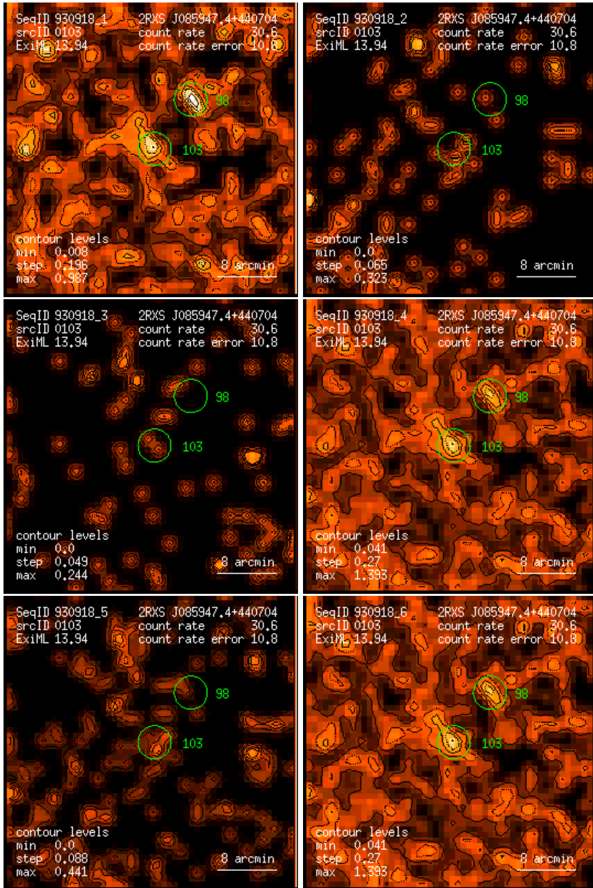
Figure 103: RASS 930918: detection 0103: band rate images, Gaussian filter: (1) PSPC channels 11 – 41, (2) 52 – 90, (3) 91 – 201, (4) 11 – 235, (5) 52 – 201, (6) 11 – 201. Broad band rates in counts/ks. Band rate contour levels in counts/ks/arcmin 2 .
