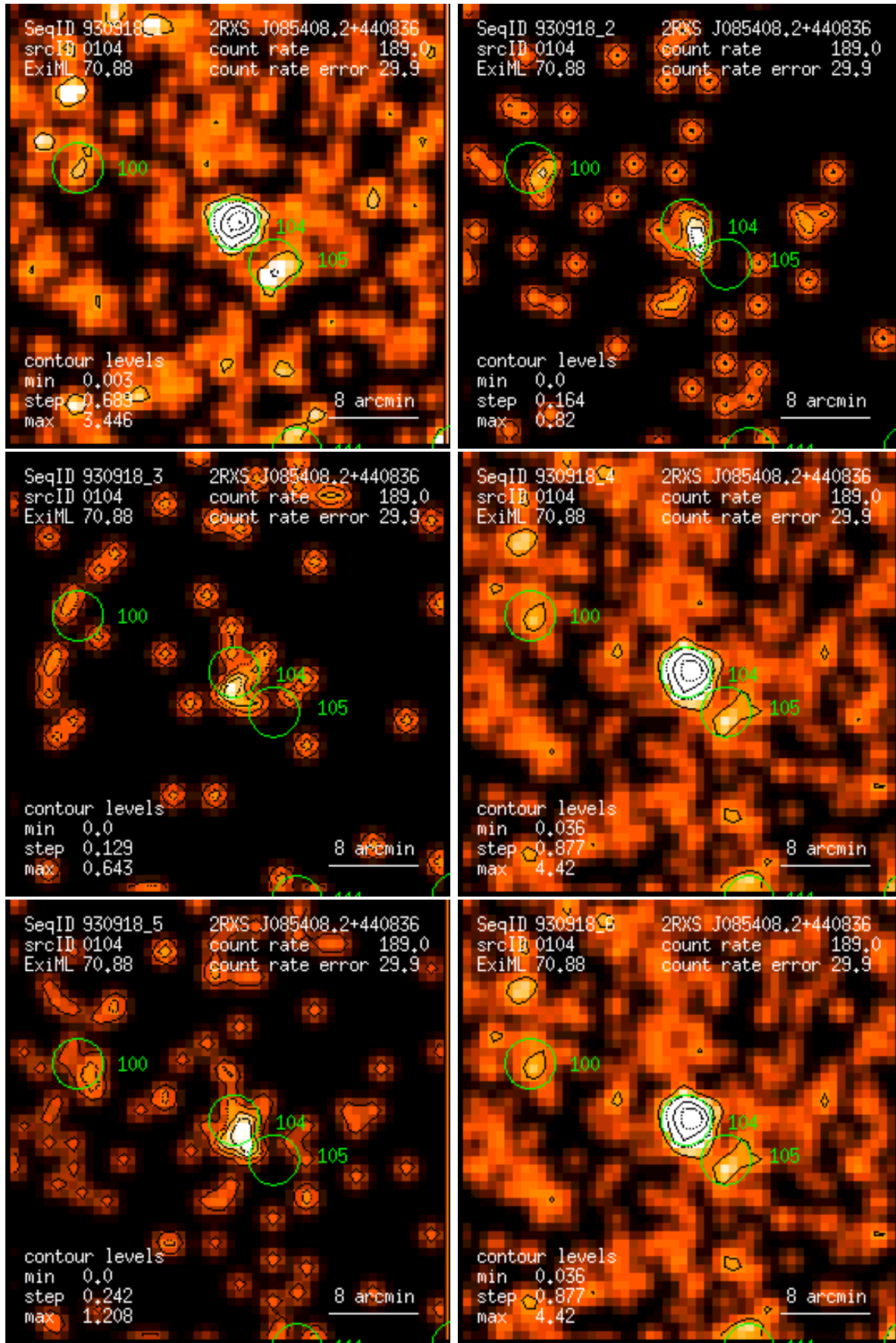
Figure 104: RASS 930918: detection 0104: band rate images, Gaussian filter: (1) PSPC channels 11 – 41, (2) 52 – 90, (3) 91 – 201, (4) 11 – 235, (5) 52 – 201, (6) 11 – 201. Broad band rates in counts/ks. Band rate contour levels in counts/ks/arcmin 2 .
