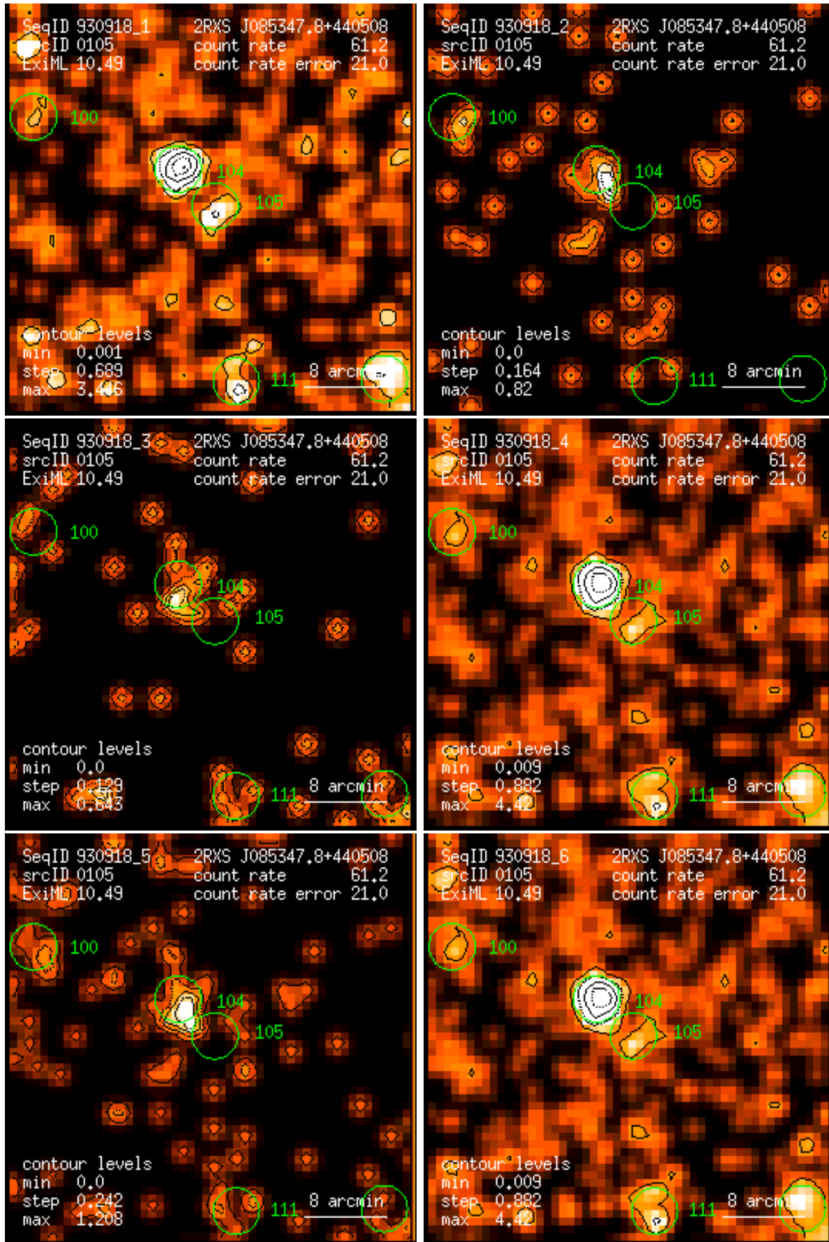
Figure 105: RASS 930918: detection 0105: band rate images, Gaussian filter: (1) PSPC channels 11 – 41, (2) 52 – 90, (3) 91 – 201, (4) 11 – 235, (5) 52 – 201, (6) 11 – 201. Broad band rates in counts/ks. Band rate contour levels in counts/ks/arcmin 2 .
