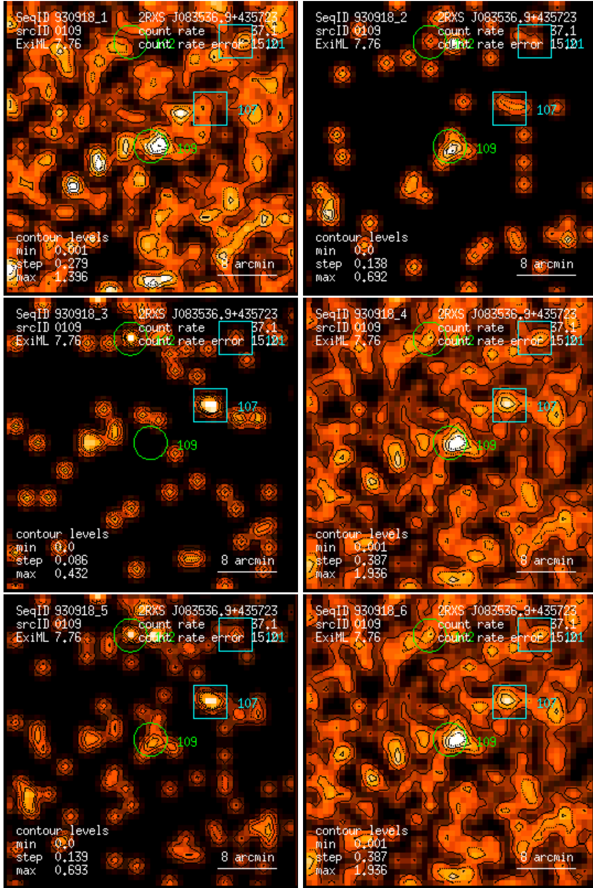
Figure 109: RASS 930918: detection 0109: band rate images, Gaussian filter: (1) PSPC channels 11 – 41, (2) 52 – 90, (3) 91 – 201, (4) 11 – 235, (5) 52 – 201, (6) 11 – 201. Broad band rates in counts/ks. Band rate contour levels in counts/ks/arcmin 2 .
