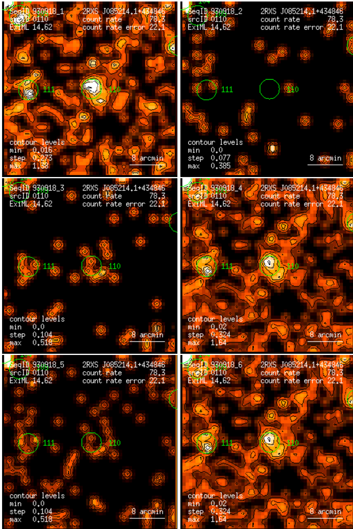
Figure 110: RASS 930918: detection 0110: band rate images, Gaussian filter: (1) PSPC channels 11 – 41, (2) 52 – 90, (3) 91 – 201, (4) 11 – 235, (5) 52 – 201, (6) 11 – 201. Broad band rates in counts/ks. Band rate contour levels in counts/ks/arcmin 2 .
