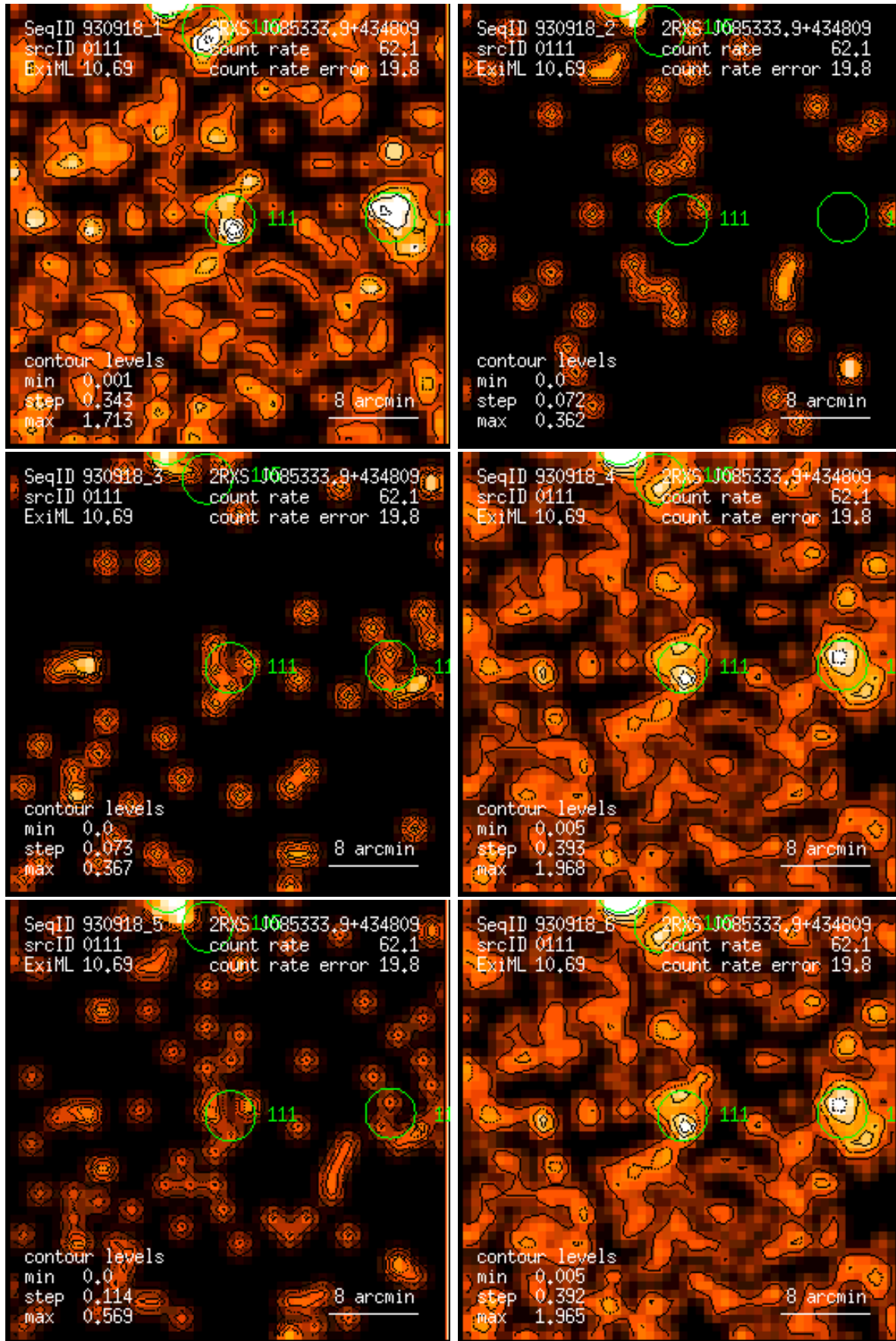
Figure 111: RASS 930918: detection 0111: band rate images, Gaussian filter: (1) PSPC channels 11 – 41, (2) 52 – 90, (3) 91 – 201, (4) 11 – 235, (5) 52 – 201, (6) 11 – 201. Broad band rates in counts/ks. Band rate contour levels in counts/ks/arcmin 2 .
