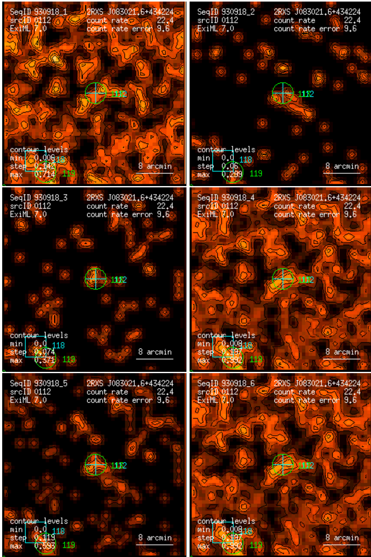
Figure 112: RASS 930918: detection 0112: band rate images, Gaussian filter: (1) PSPC channels 11 – 41, (2) 52 – 90, (3) 91 – 201, (4) 11 – 235, (5) 52 – 201, (6) 11 – 201. Broad band rates in counts/ks. Band rate contour levels in counts/ks/arcmin 2 .
