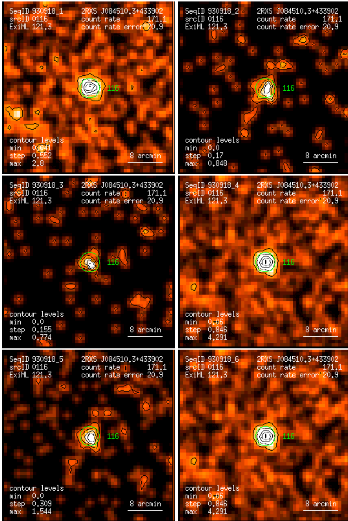
Figure 116: RASS 930918: detection 0116: band rate images, Gaussian filter: (1) PSPC channels 11 – 41, (2) 52 – 90, (3) 91 – 201, (4) 11 – 235, (5) 52 – 201, (6) 11 – 201. Broad band rates in counts/ks. Band rate contour levels in counts/ks/arcmin 2 .
