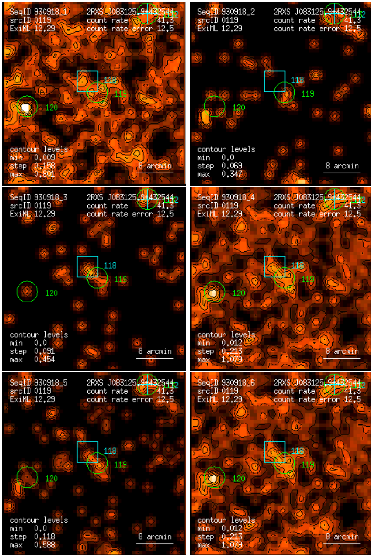
Figure 119: RASS 930918: detection 0119: band rate images, Gaussian filter: (1) PSPC channels 11 – 41, (2) 52 – 90, (3) 91 – 201, (4) 11 – 235, (5) 52 – 201, (6) 11 – 201. Broad band rates in counts/ks. Band rate contour levels in counts/ks/arcmin 2 .
