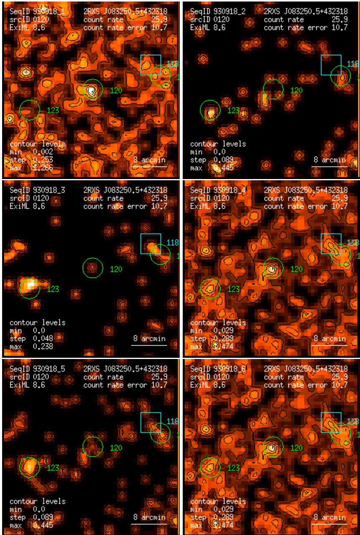
Figure 120: RASS 930918: detection 0120: band rate images, Gaussian filter: (1) PSPC channels 11 – 41, (2) 52 – 90, (3) 91 – 201, (4) 11 – 235, (5) 52 – 201, (6) 11 – 201. Broad band rates in counts/ks. Band rate contour levels in counts/ks/arcmin 2 .
