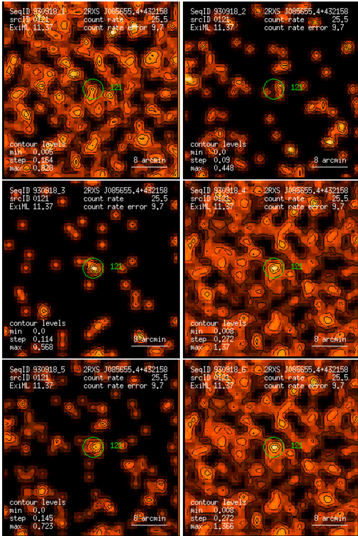
Figure 121: RASS 930918: detection 0121: band rate images, Gaussian filter: (1) PSPC channels 11 – 41, (2) 52 – 90, (3) 91 – 201, (4) 11 – 235, (5) 52 – 201, (6) 11 – 201. Broad band rates in counts/ks. Band rate contour levels in counts/ks/arcmin 2 .
