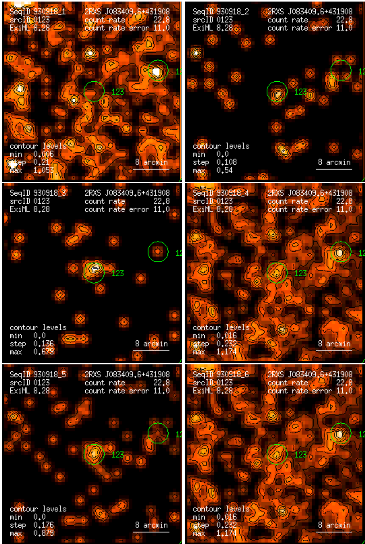
Figure 123: RASS 930918: detection 0123: band rate images, Gaussian filter: (1) PSPC channels 11 – 41, (2) 52 – 90, (3) 91 – 201, (4) 11 – 235, (5) 52 – 201, (6) 11 – 201. Broad band rates in counts/ks. Band rate contour levels in counts/ks/arcmin 2 .
