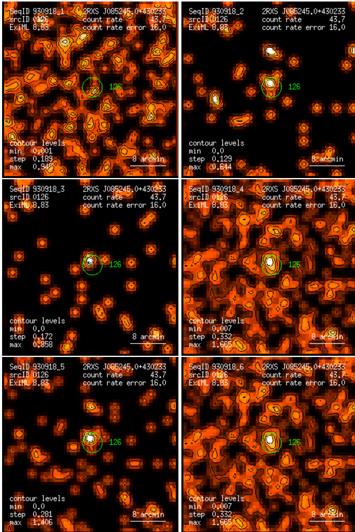
Figure 126: RASS 930918: detection 0126: band rate images, Gaussian filter: (1) PSPC channels 11 – 41, (2) 52 – 90, (3) 91 – 201, (4) 11 – 235, (5) 52 – 201, (6) 11 – 201. Broad band rates in counts/ks. Band rate contour levels in counts/ks/arcmin 2 .
