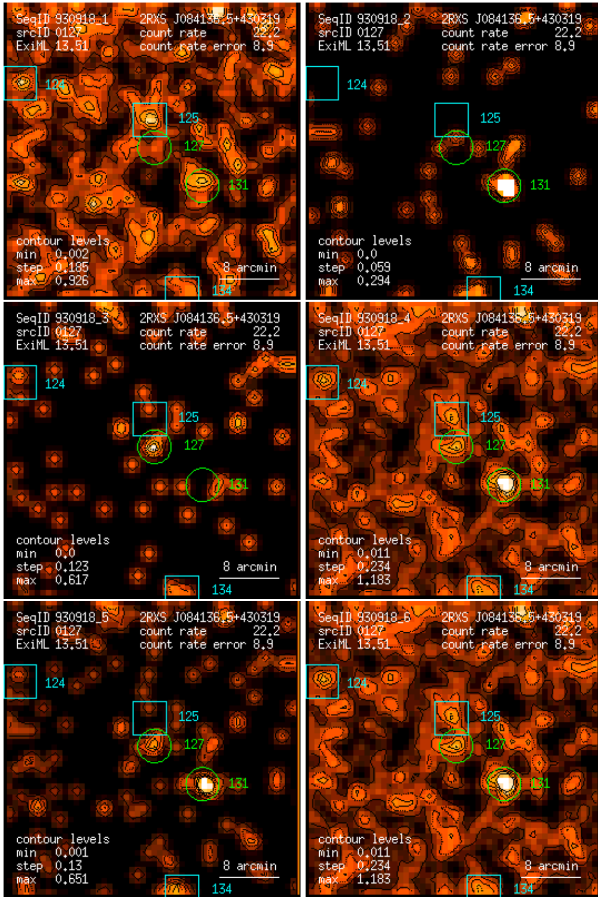
Figure 127: RASS 930918: detection 0127: band rate images, Gaussian filter: (1) PSPC channels 11 – 41, (2) 52 – 90, (3) 91 – 201, (4) 11 – 235, (5) 52 – 201, (6) 11 – 201. Broad band rates in counts/ks. Band rate contour levels in counts/ks/arcmin 2 .
