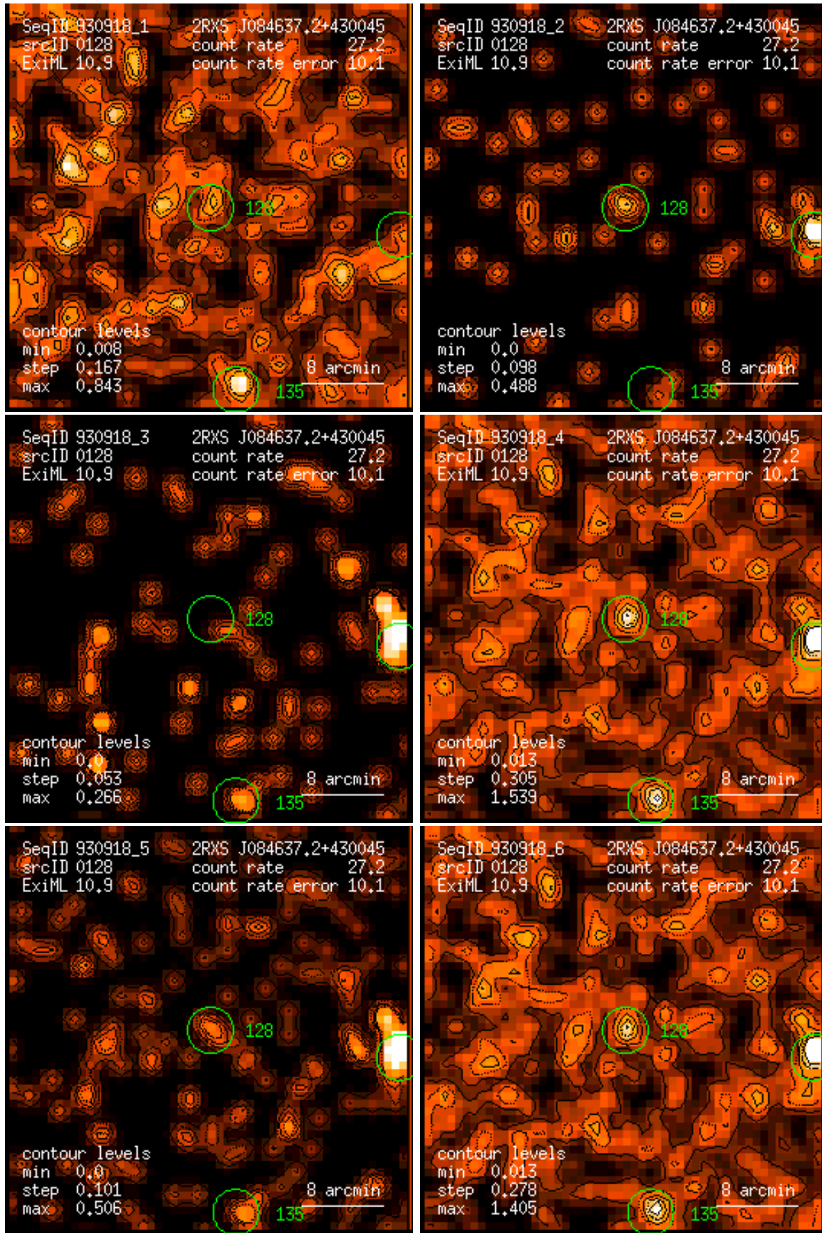
Figure 128: RASS 930918: detection 0128: band rate images, Gaussian filter: (1) PSPC channels 11 – 41, (2) 52 – 90, (3) 91 – 201, (4) 11 – 235, (5) 52 – 201, (6) 11 – 201. Broad band rates in counts/ks. Band rate contour levels in counts/ks/arcmin 2 .
