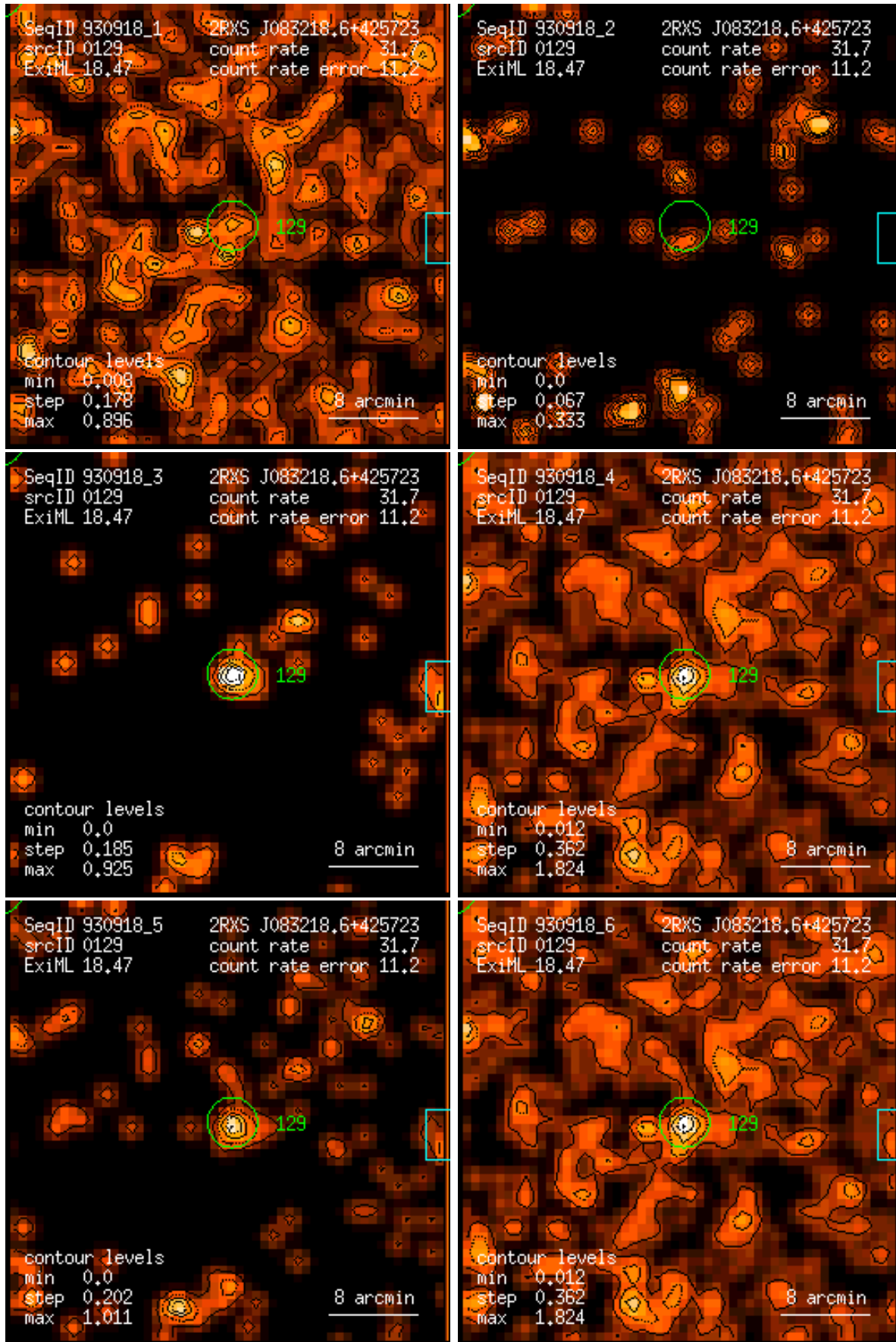
Figure 129: RASS 930918: detection 0129: band rate images, Gaussian filter: (1) PSPC channels 11 – 41, (2) 52 – 90, (3) 91 – 201, (4) 11 – 235, (5) 52 – 201, (6) 11 – 201. Broad band rates in counts/ks. Band rate contour levels in counts/ks/arcmin 2 .
