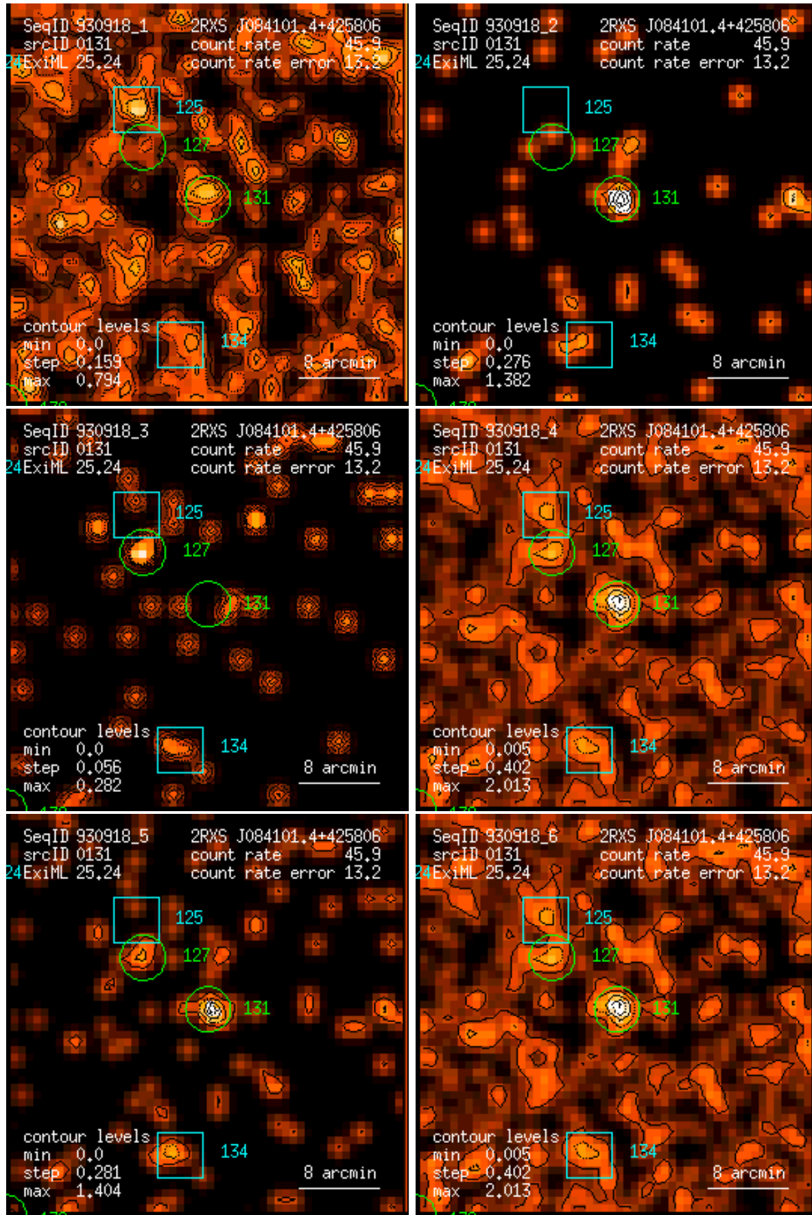
Figure 131: RASS 930918: detection 0131: band rate images, Gaussian filter: (1) PSPC channels 11 – 41, (2) 52 – 90, (3) 91 – 201, (4) 11 – 235, (5) 52 – 201, (6) 11 – 201. Broad band rates in counts/ks. Band rate contour levels in counts/ks/arcmin 2 .
